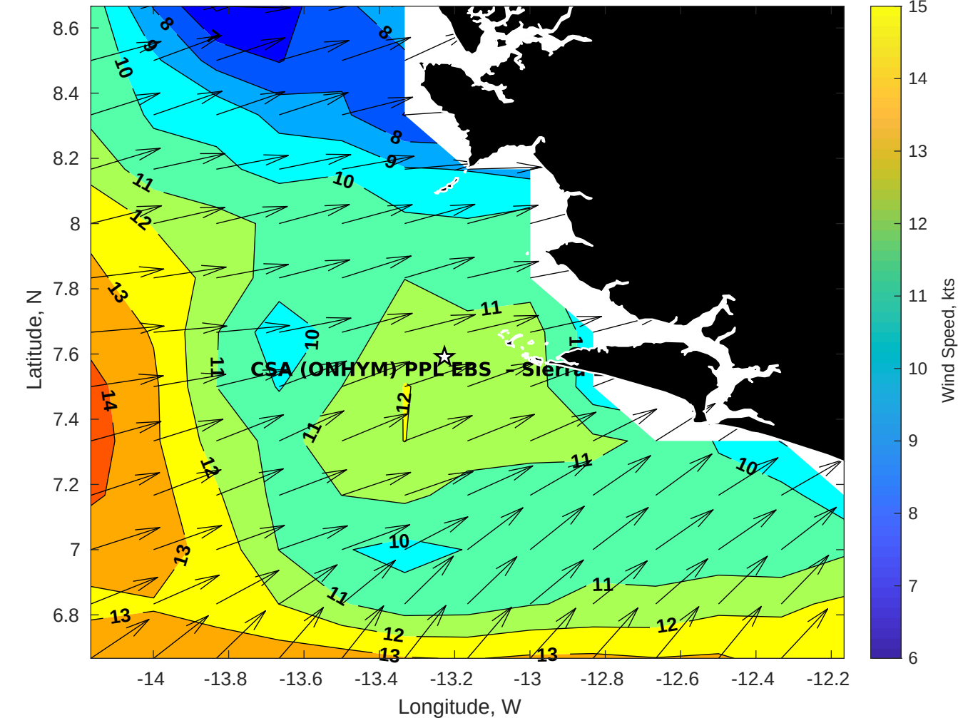
Winds (kts) for CSA (ONHYM) PPL EBS - Sierra Leone at 11-Sep-2025 09:00:00
