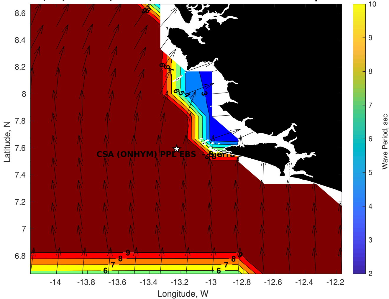
Wave Period (sec) for CSA (ONHYM) PPL EBS - Sierra Leone at 11-Sep-2025 09:00:00
