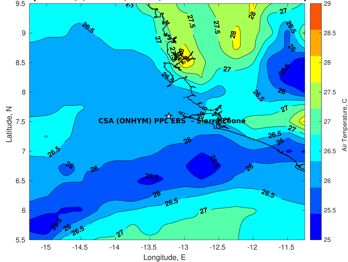
Air Temperature (C) for CSA (ONHYM) PPL EBS - Sierra Leone at 10-Sep-2025
