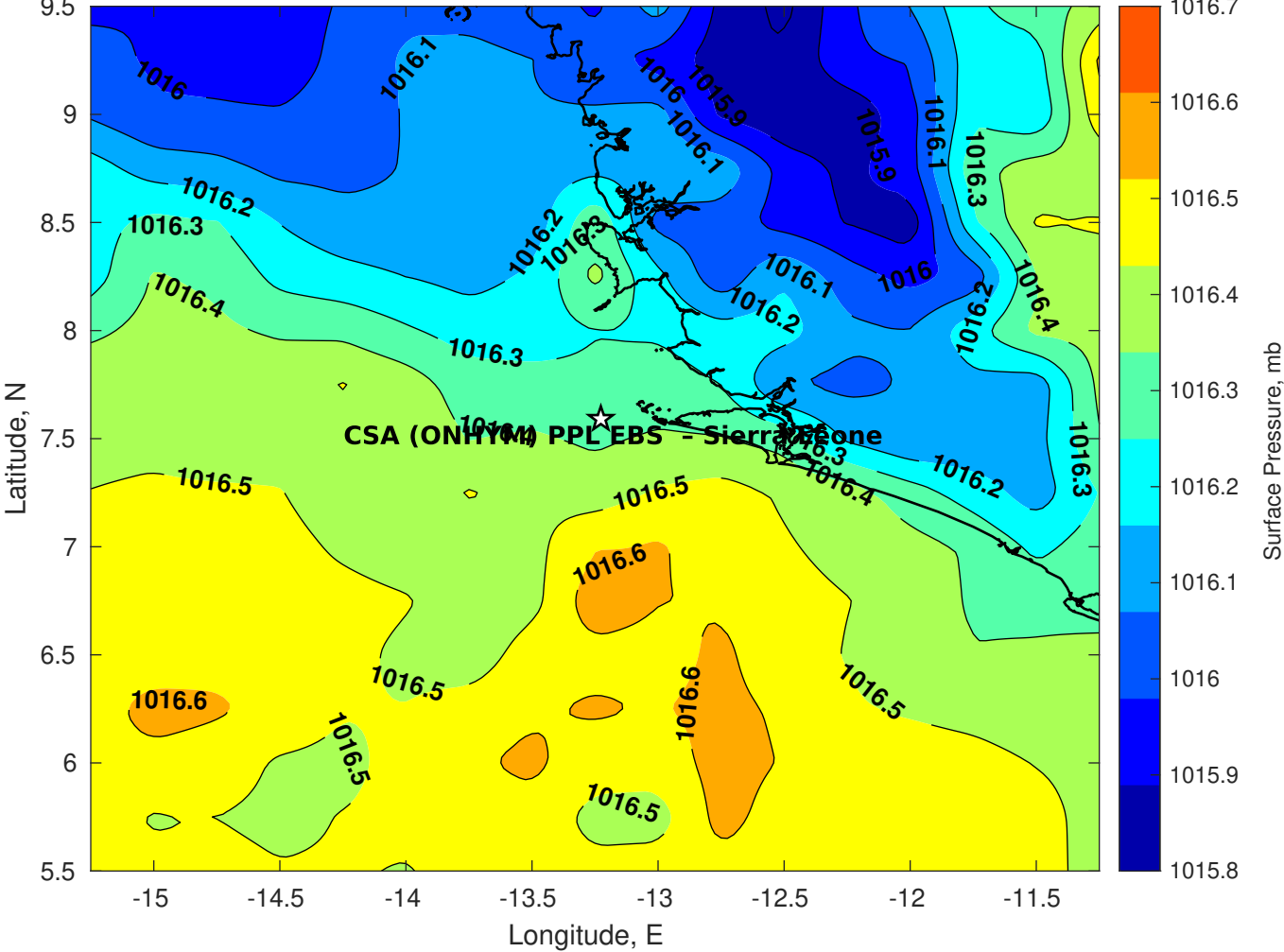
Surface Pressure (mb) for CSA (ONHYM) PPL EBS - Sierra Leone at 11-Sep-2025 12:00:00
