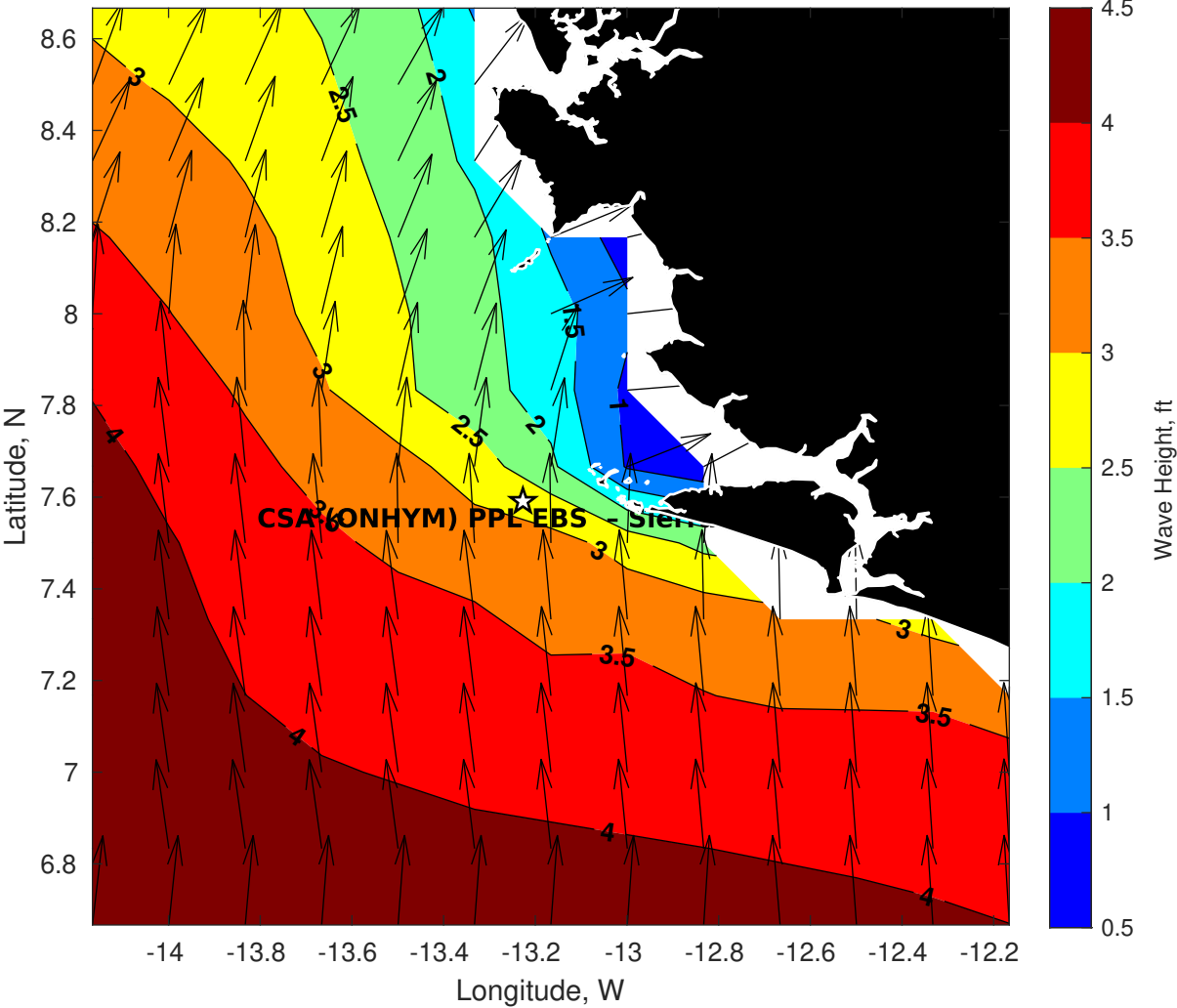
Wave Height (ft) for CSA (ONHYM) PPL EBS - Sierra Leone at 11-Sep-2025 09:00:00
