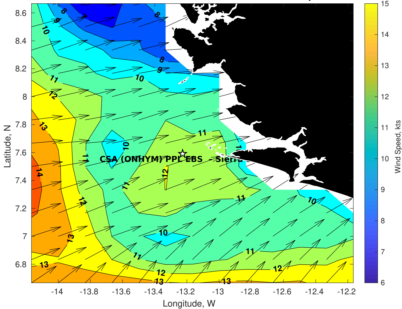
Winds (kts) for CSA (ONHYM) PPL EBS - Sierra Leone at 11-Sep-2025 09:00:00
