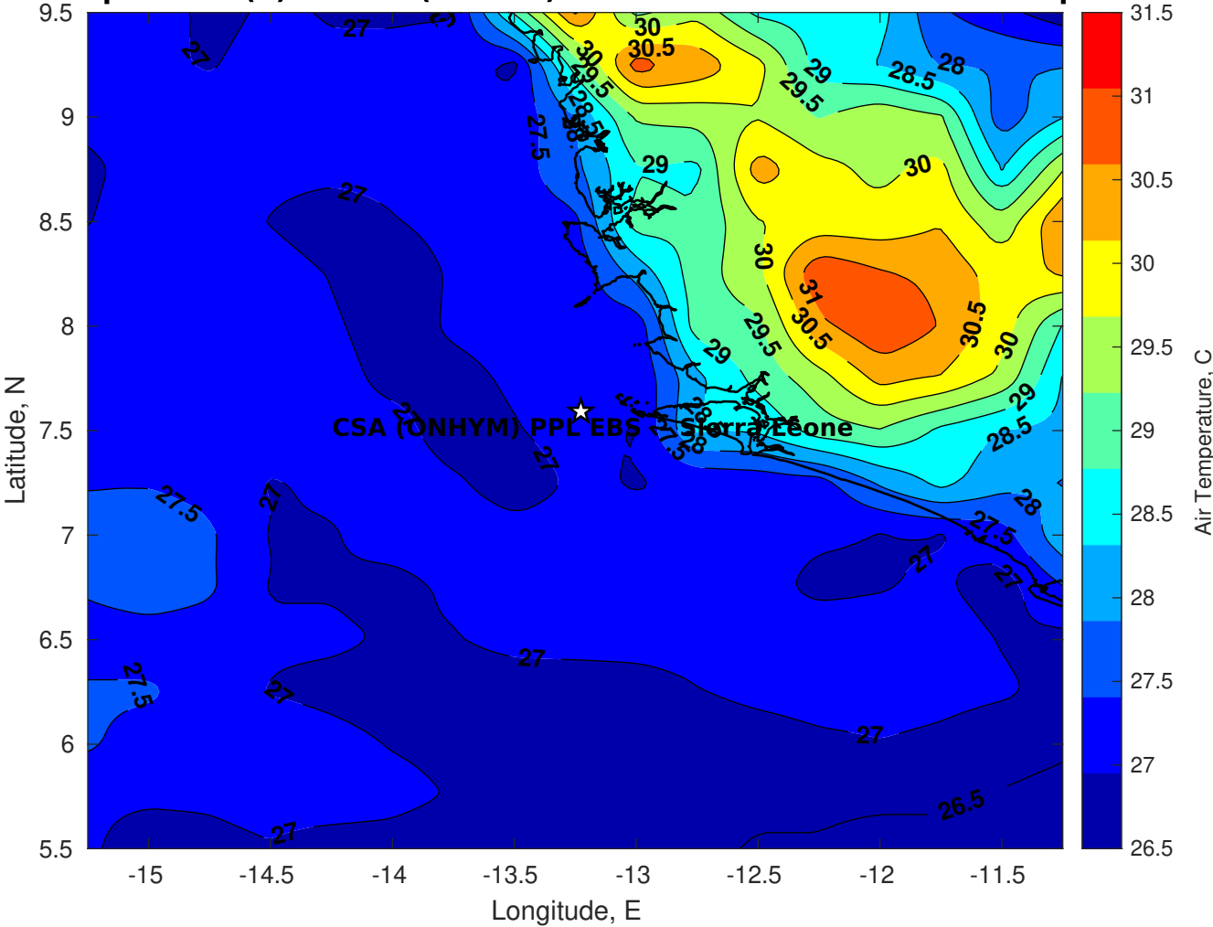
Air Temperature (C) for CSA (ONHYM) PPL EBS - Sierra Leone at 10-Sep-2025
