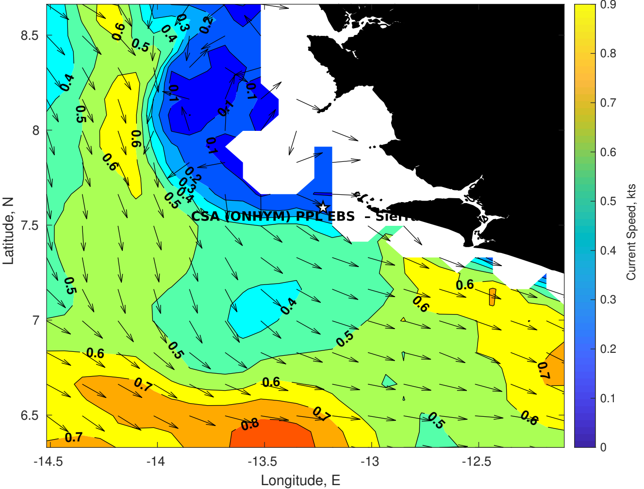
Surface Currents for CSA (ONHYM) PPL EBS - Sierra Leone at 10-Sep-2025 00:00:00
