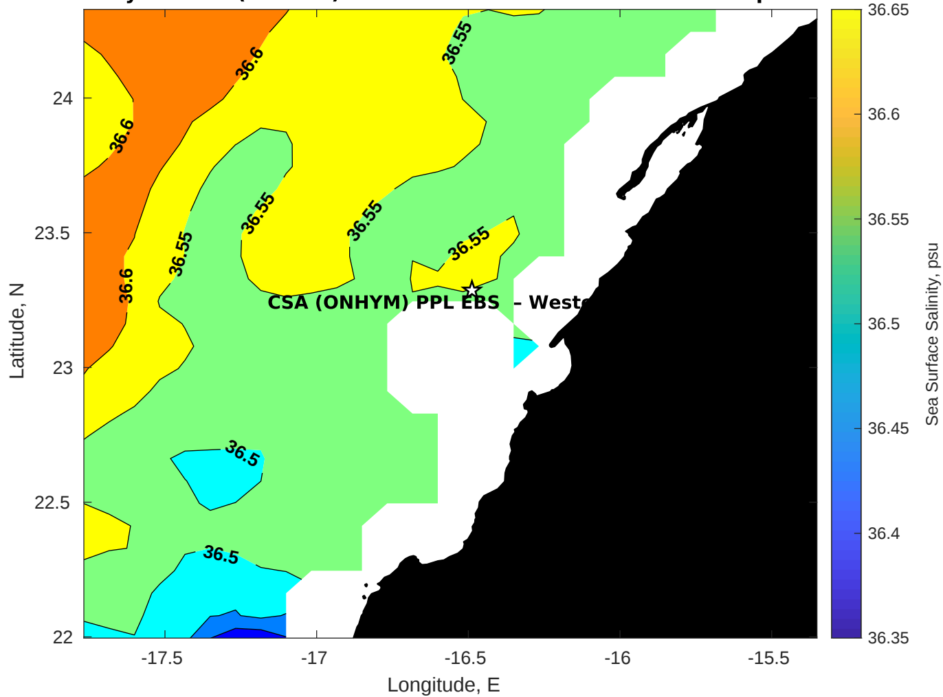
Surface Salinity for CSA (ONHYM) PPL EBS - Western Sahara at 10-Sep-2025 00:00:00
