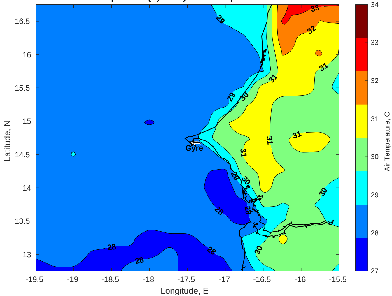
Air Temperature (C) for Gyre at 10-Sep-2025
