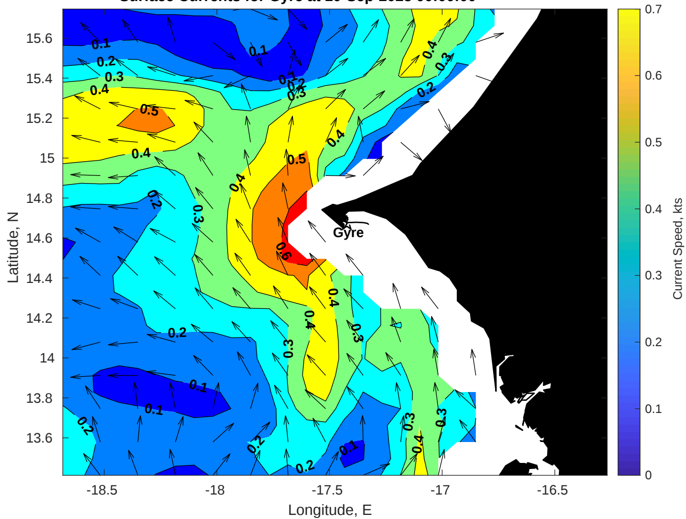
Surface Currents for Gyre at 10-Sep-2025 00:00:00
