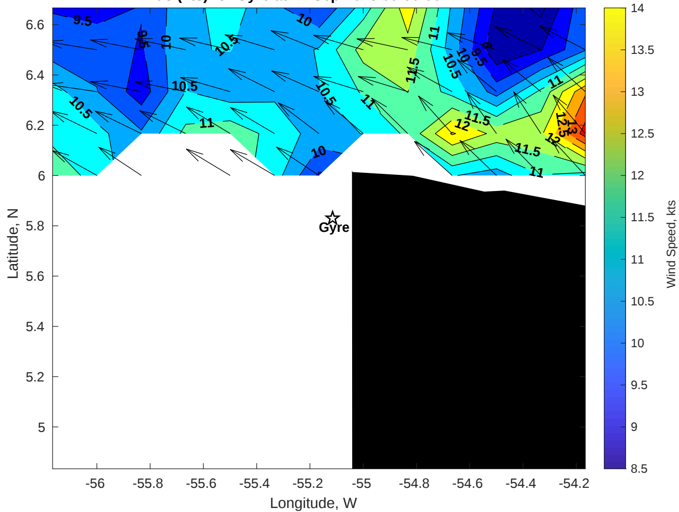
Winds (kts) for Gyre at 11-Sep-2025 09:00:00
