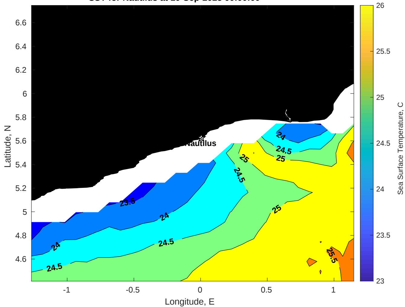
SST for Nautilus at 10-Sep-2025 00:00:00
