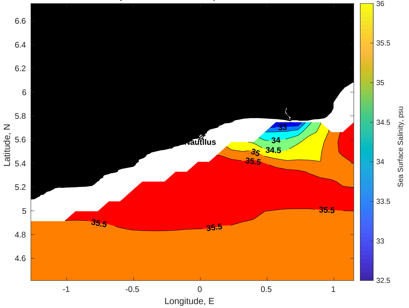
Surface Salinity for Nautilus at 10-Sep-2025 00:00:00
