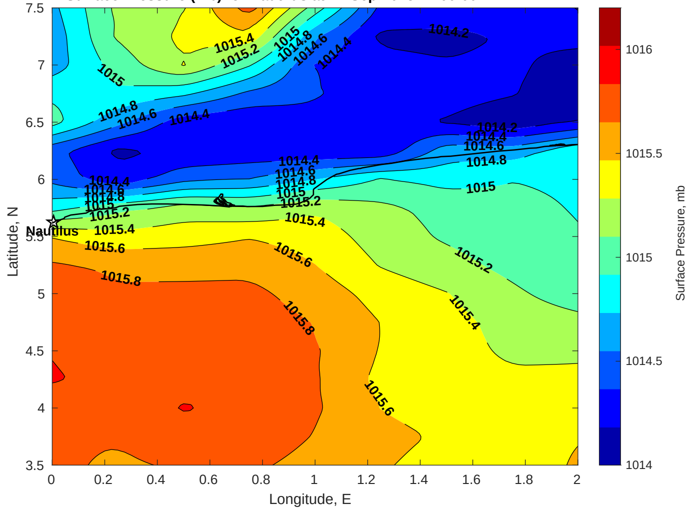
Surface Pressure (mb) for Nautilus at 11-Sep-2025 12:00:00
