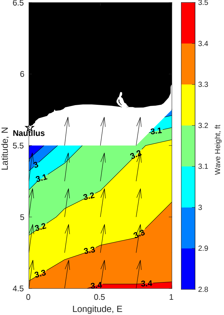
Wave Height (ft) for Nautilus at 11-Sep-2025 09:00:00
