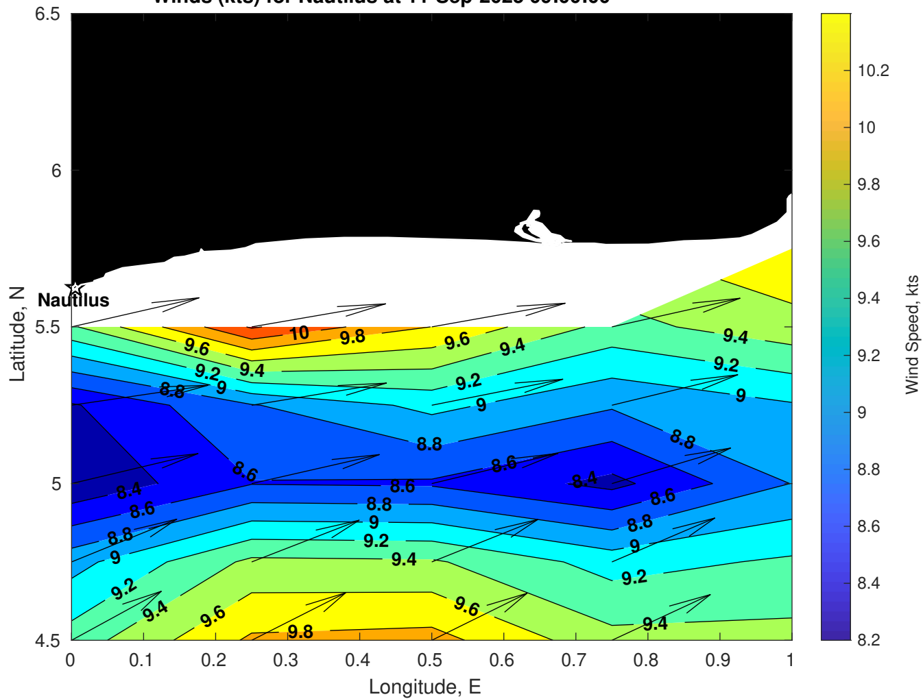
Winds (kts) for Nautilus at 11-Sep-2025 09:00:00
