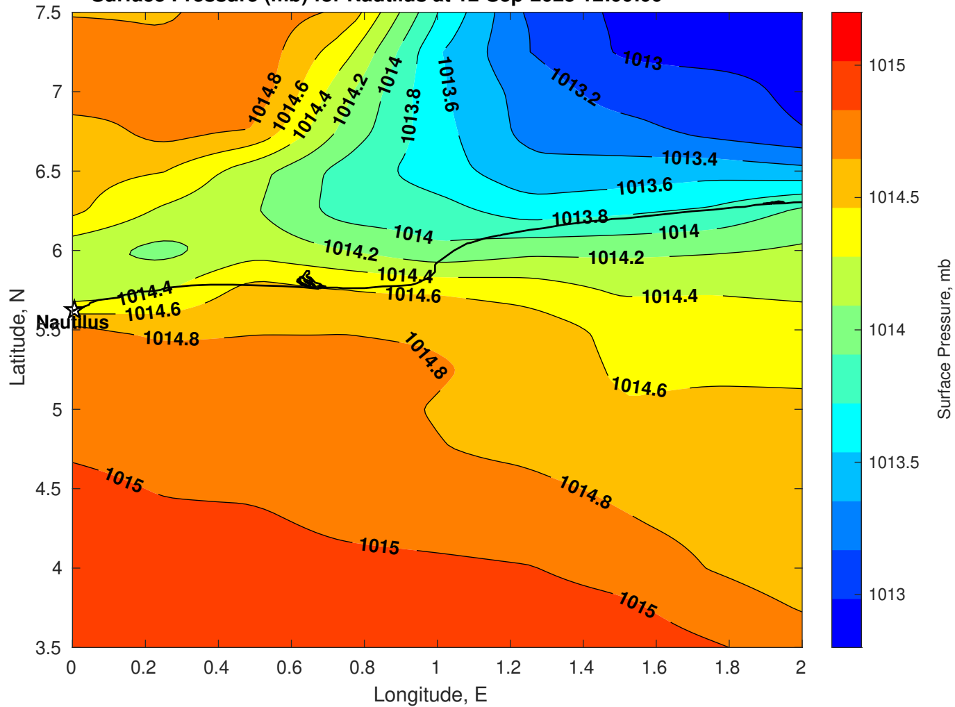
Surface Pressure (mb) for Nautilus at 12-Sep-2025 12:00:00
