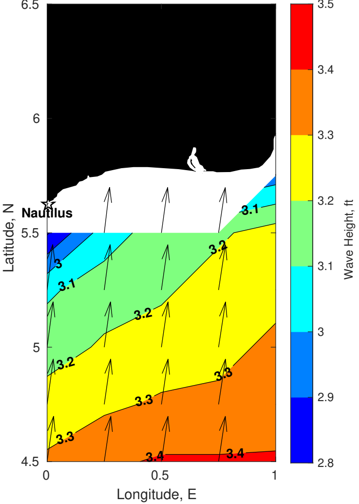
Wave Height (ft) for Nautilus at 11-Sep-2025 09:00:00
