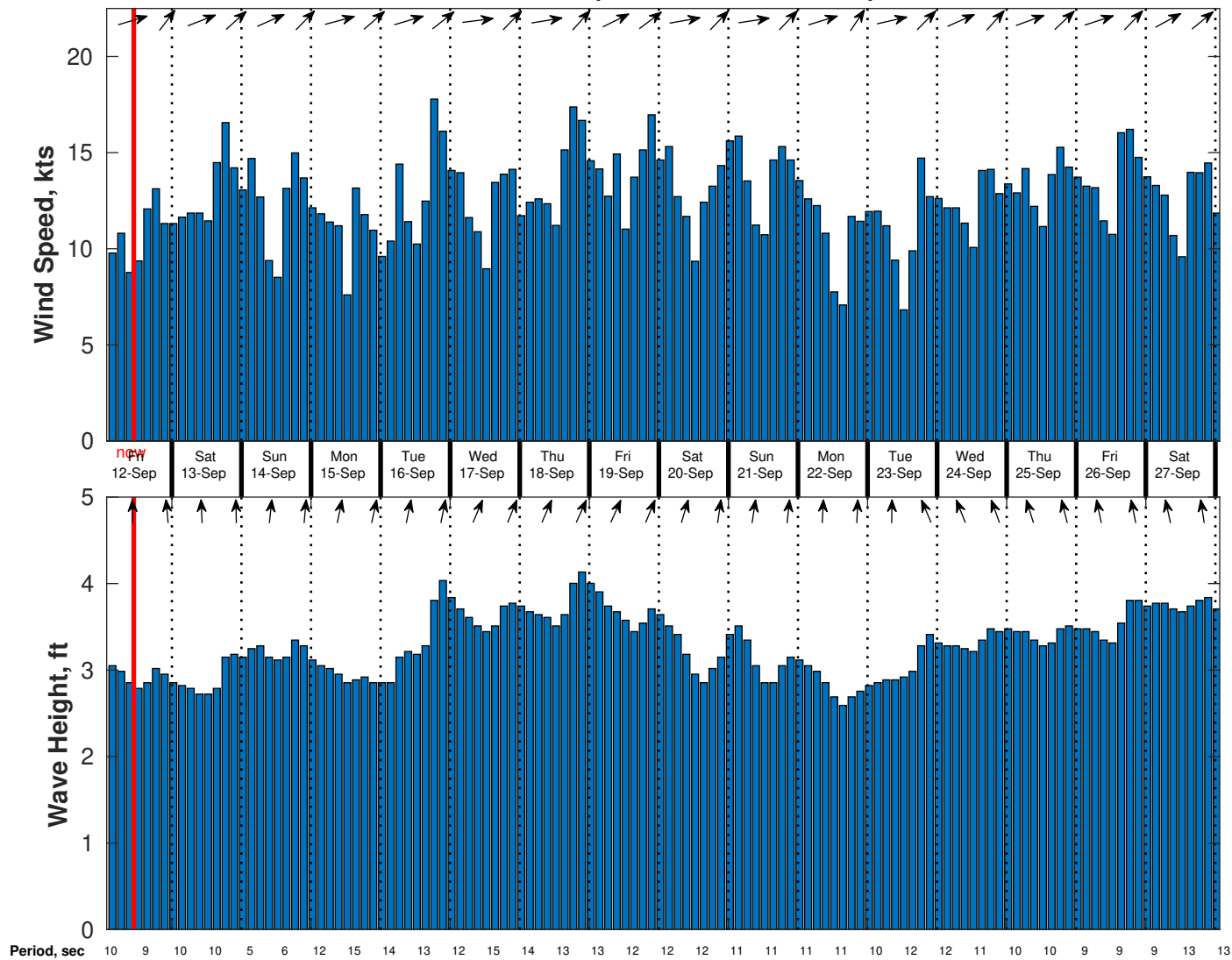
Wind & Wave Forecast for Nautilus from 11-Sep-2025 02:00:00 to 27-Sep-2025 02:00:00
