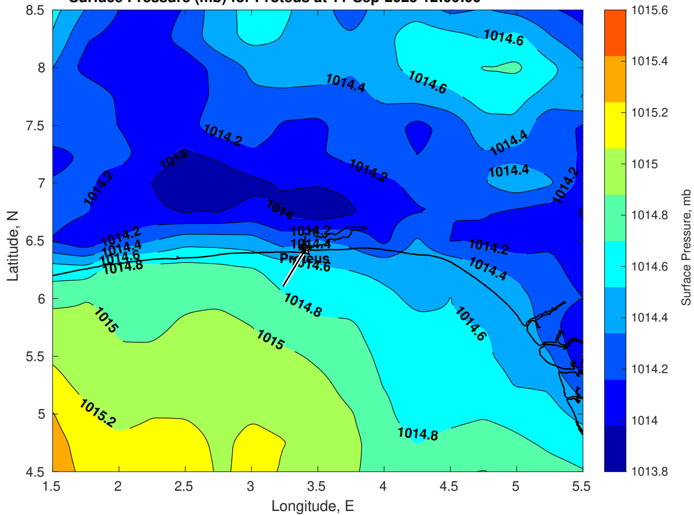
Surface Pressure (mb) for Proteus at 11-Sep-2025 12:00:00
