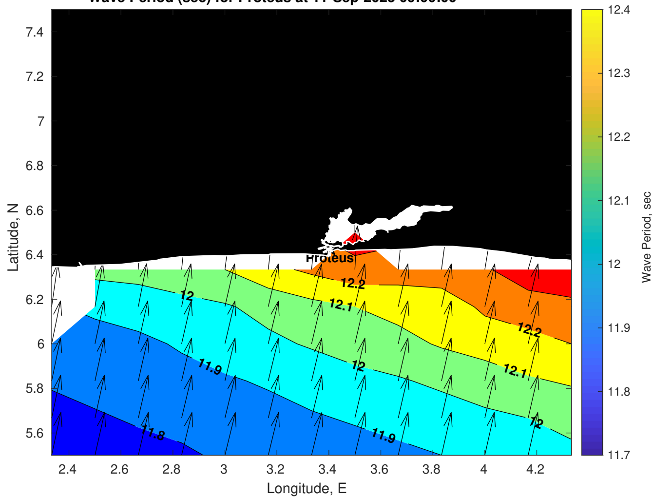
Wave Period (sec) for Proteus at 11-Sep-2025 09:00:00
