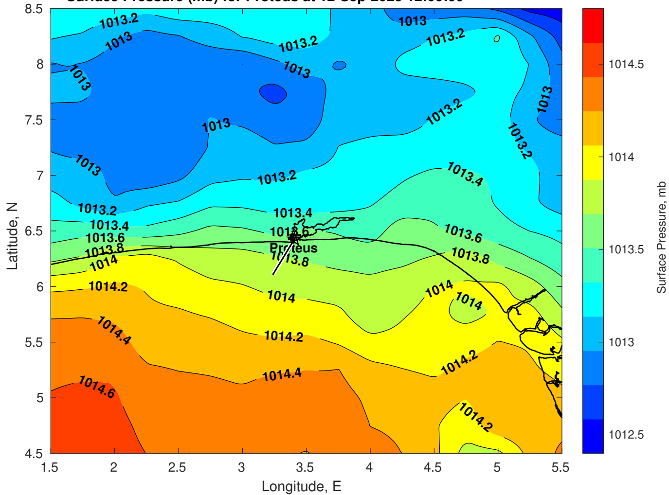
Surface Pressure (mb) for Proteus at 12-Sep-2025 12:00:00
