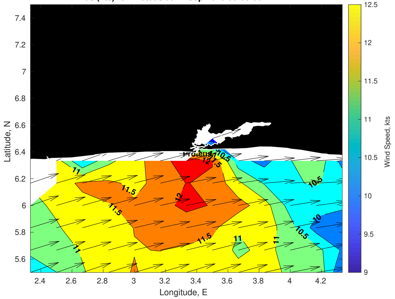
Winds (kts) for Proteus at 11-Sep-2025 09:00:00
