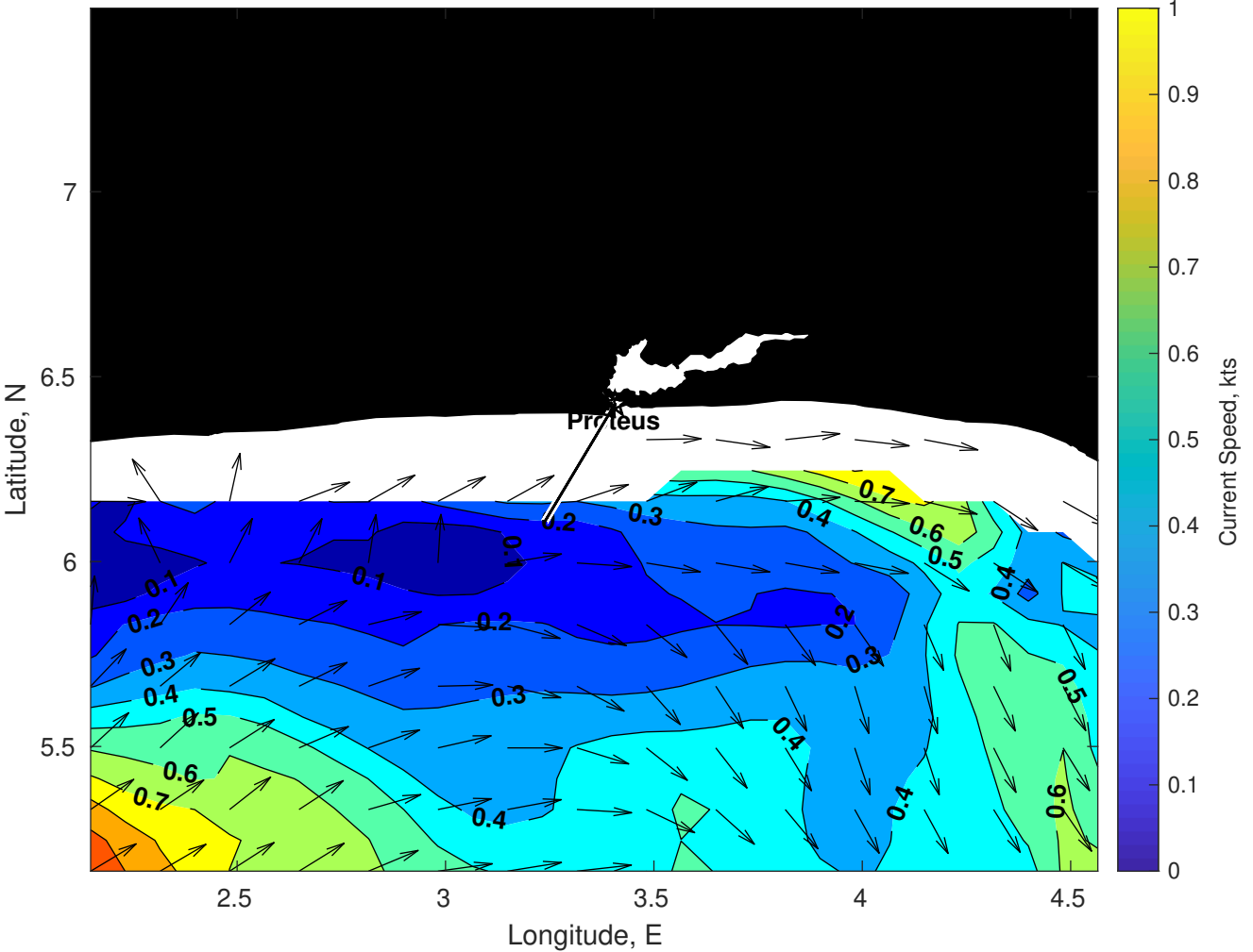
Surface Currents for Proteus at 10-Sep-2025 00:00:00
