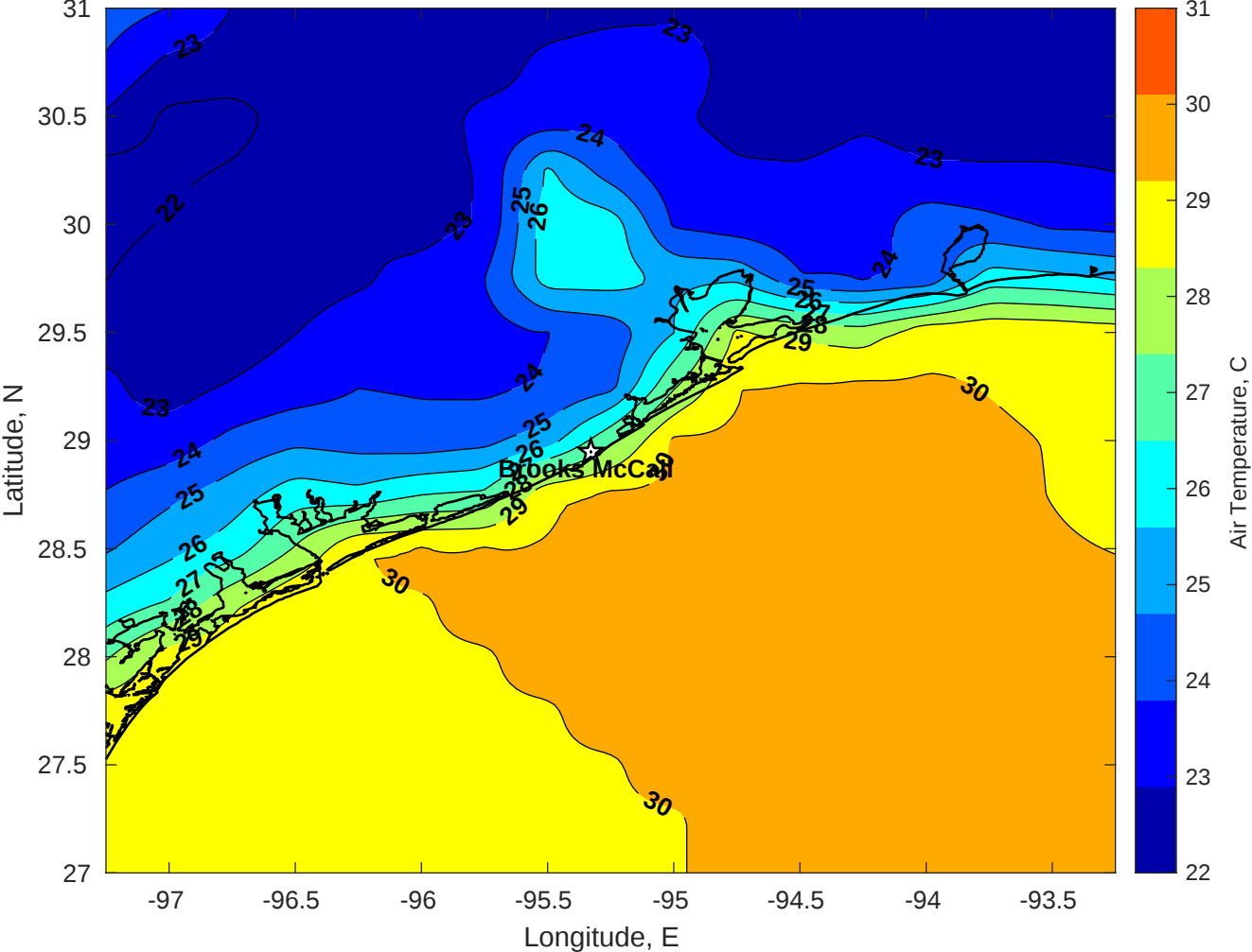
Air Temperature (C) for Brooks McCall at 11-Sep-2025
