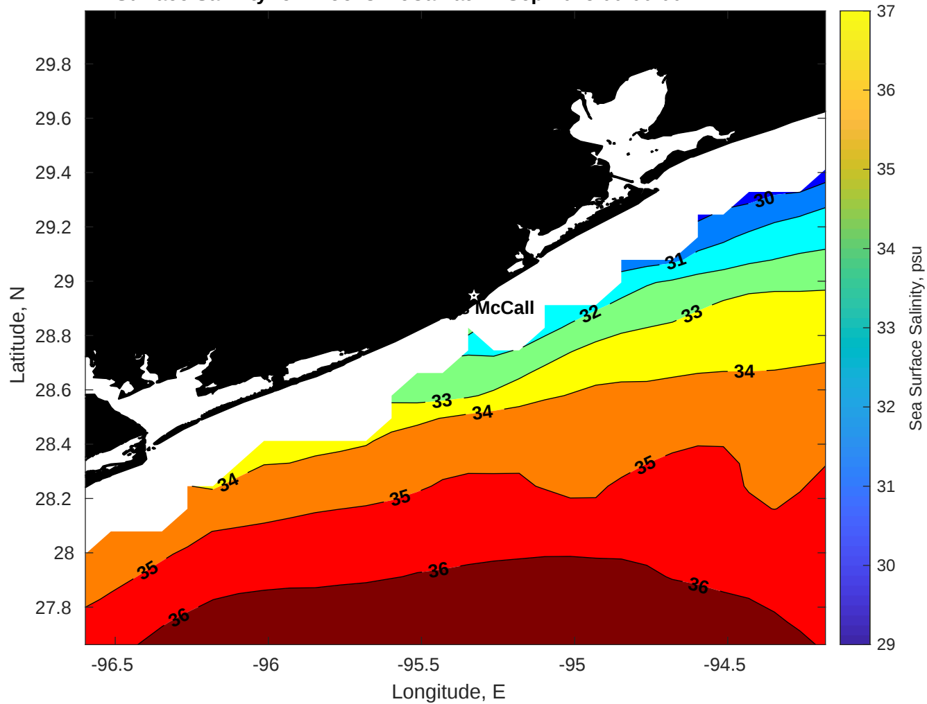
Surface Salinity for Brooks McCall at 11-Sep-2025 00:00:00
