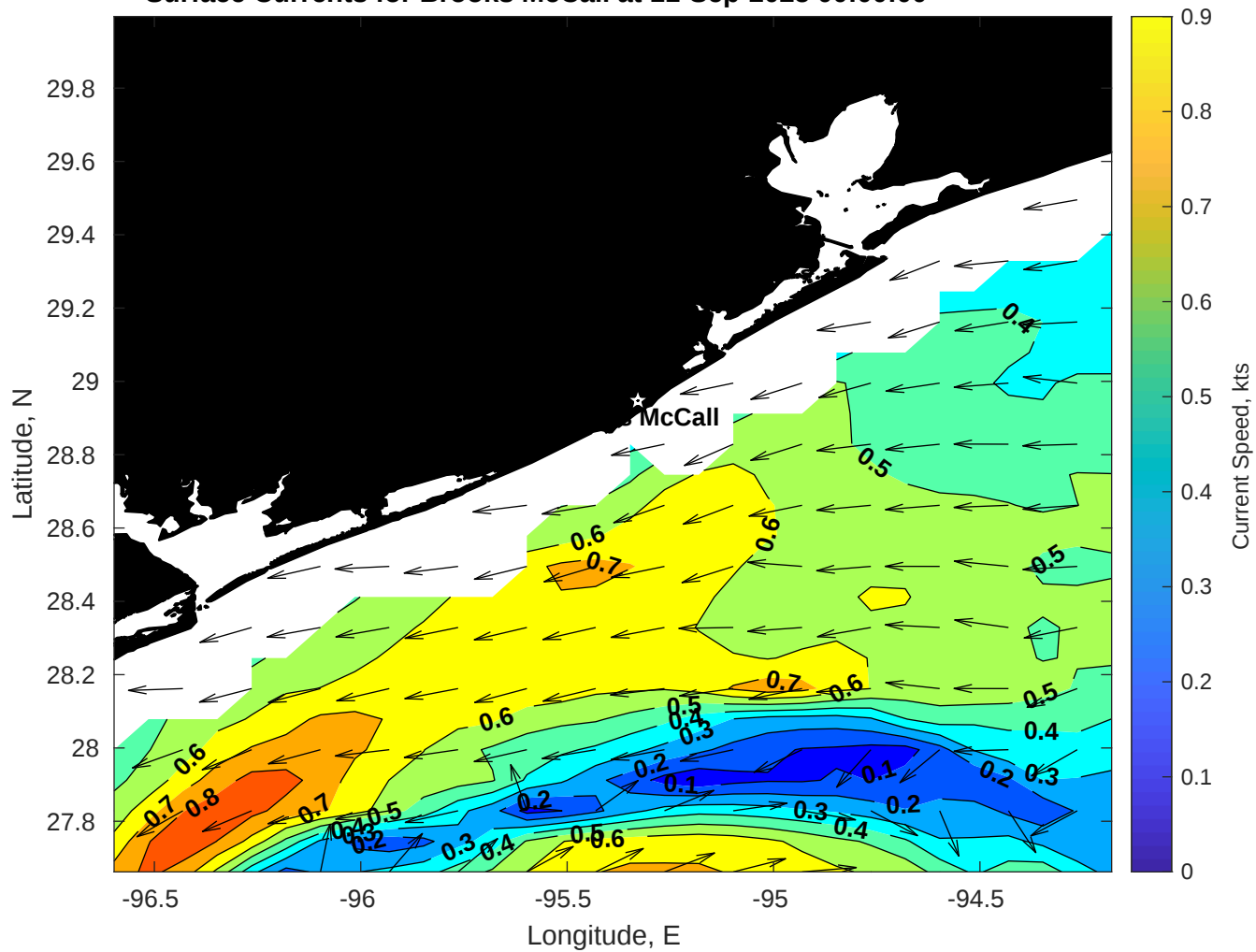
Surface Currents for Brooks McCall at 11-Sep-2025 00:00:00
