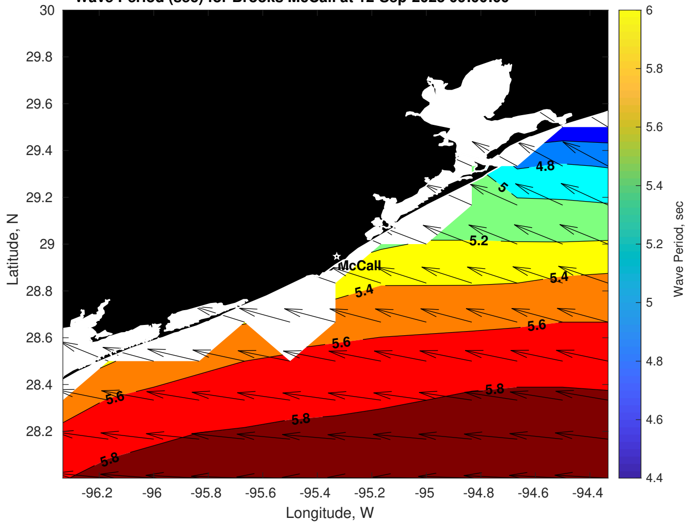
Wave Period (sec) for Brooks McCall at 12-Sep-2025 09:00:00
