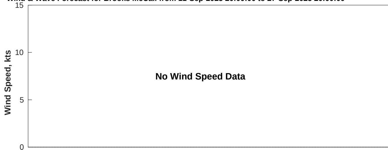
Wind & Wave Forecast for Brooks McCall from 11-Sep-2025 20:00:00 to 27-Sep-2025 20:00:00
