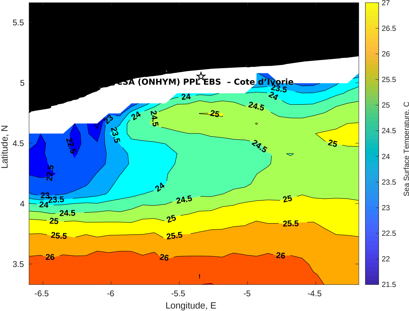
SST for CSA (ONHYM) PPL EBS - Cote d'Ivoire at 11-Sep-2025 00:00:00
