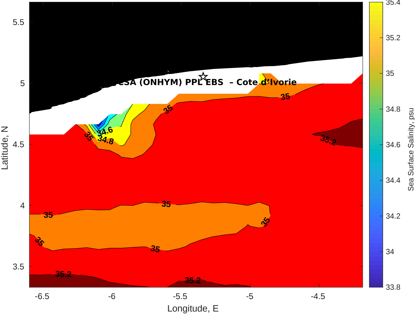
Surface Salinity for CSA (ONHYM) PPL EBS - Cote d'Ivoire at 11-Sep-2025 00:00:00
