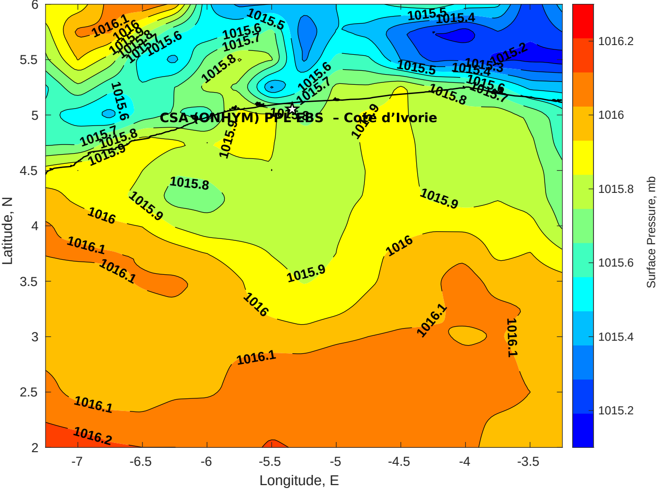
Surface Pressure (mb) for CSA (ONHYM) PPL EBS - Cote d'Ivoire at 13-Sep-2025 12:00:00
