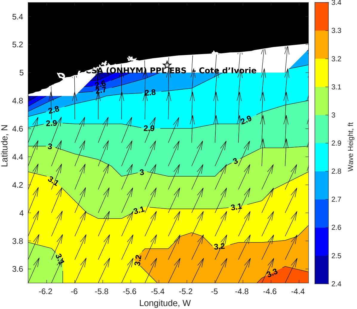
Wave Height (ft) for CSA (ONHYM) PPL EBS - Cote d'Ivoire at 12-Sep-2025 09:00:00
