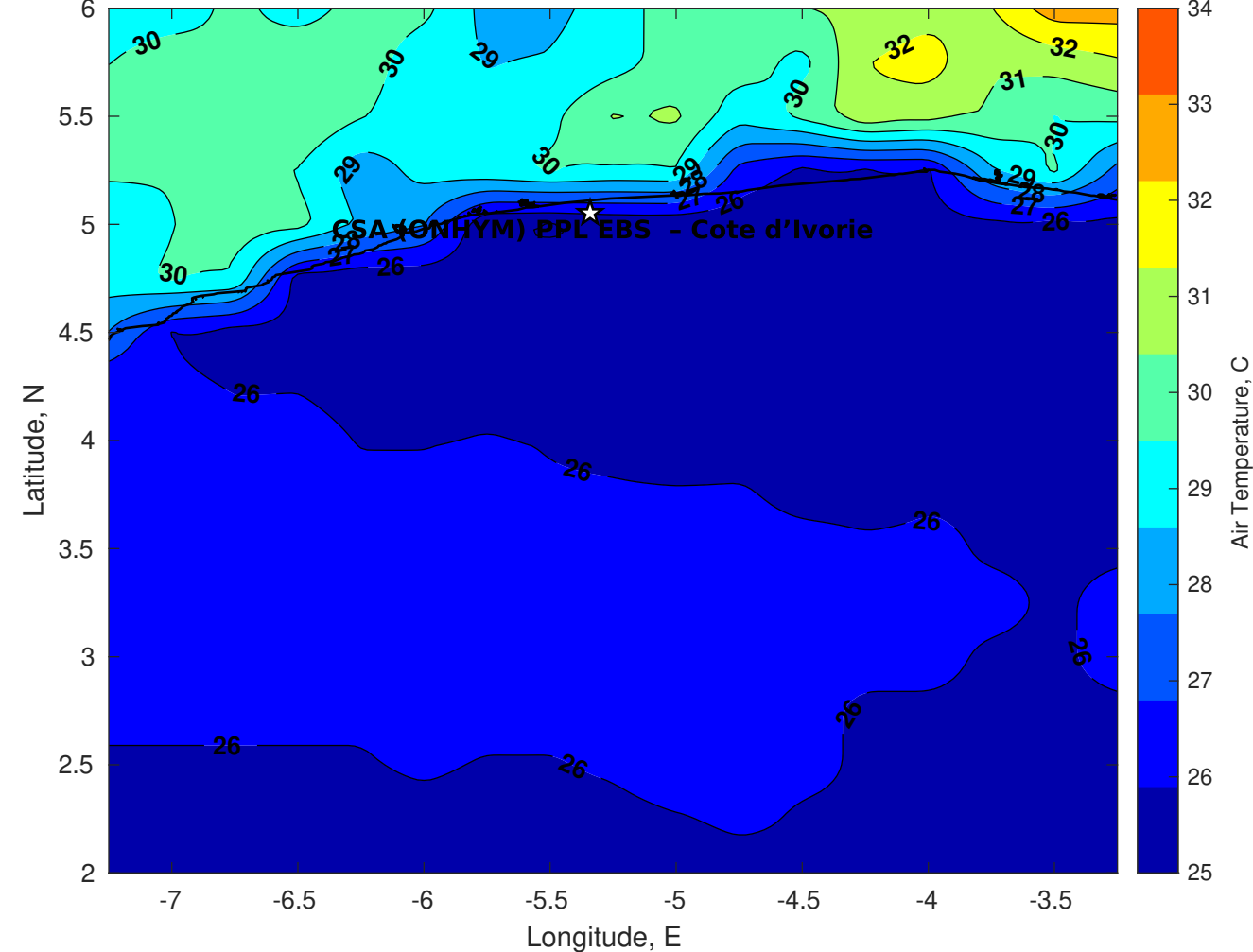
Air Temperature (C) for CSA (ONHYM) PPL EBS - Cote d'Ivoire at 11-Sep-2025
