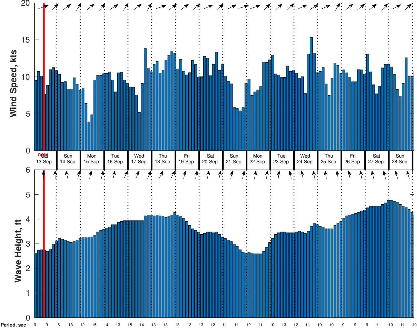
Wind & Wave Forecast for CSA (ONHYM) PPL EBS - Cote d'Ivoire from 12-Sep-2025 01:00:00 to 28-Sep-2025 01:00:00
