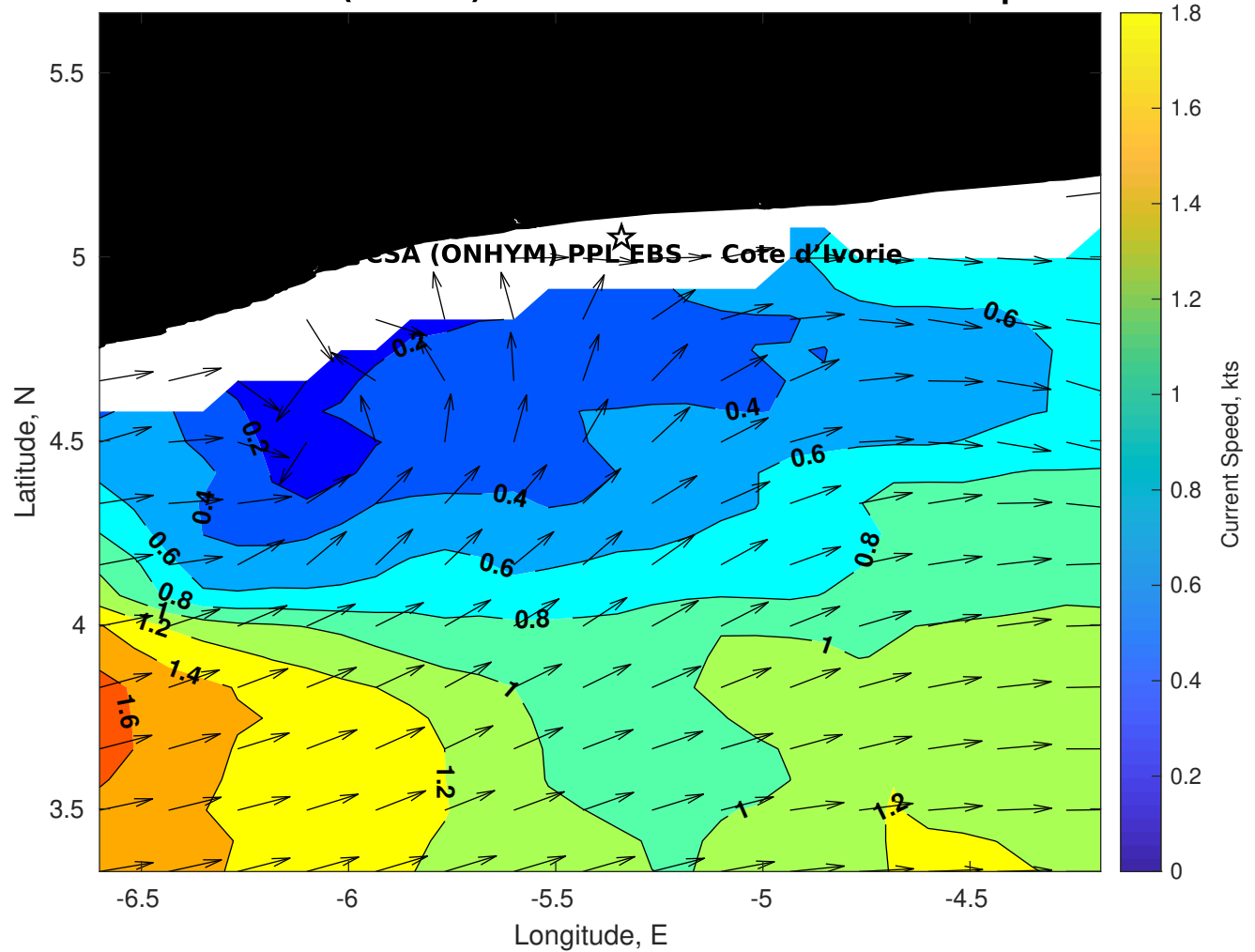
Surface Currents for CSA (ONHYM) PPL EBS - Cote d'Ivoire at 11-Sep-2025 00:00:00
