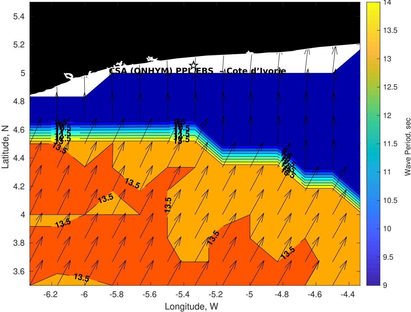
Wave Period (sec) for CSA (ONHYM) PPL EBS - Cote d'Ivoire at 12-Sep-2025 09:00:00
