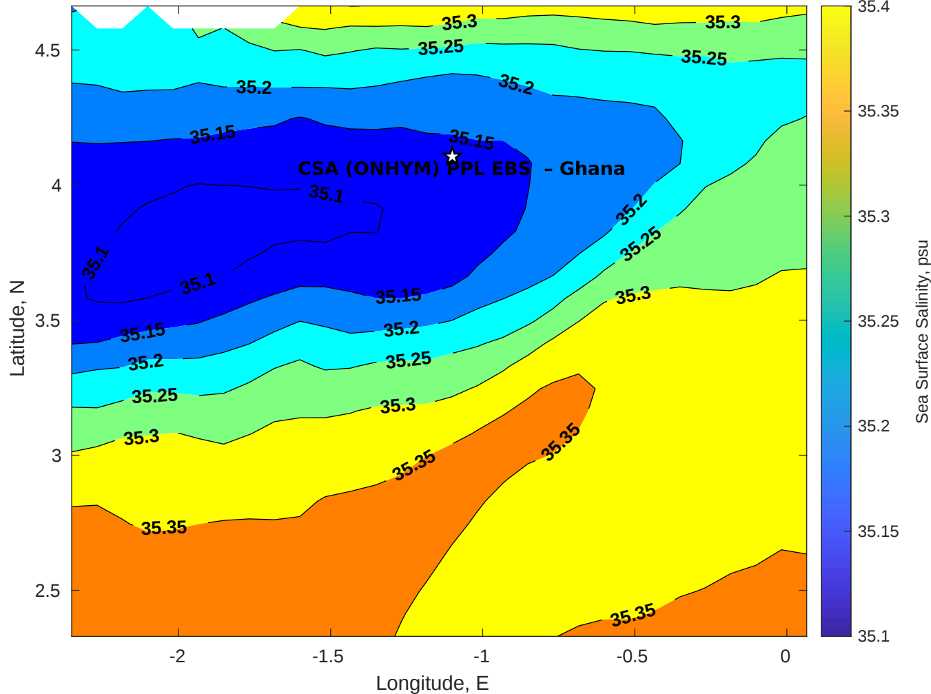
Surface Salinity for CSA (ONHYM) PPL EBS - Ghana at 11-Sep-2025 00:00:00
