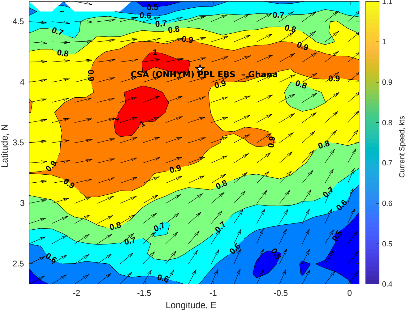
Surface Currents for CSA (ONHYM) PPL EBS - Ghana at 11-Sep-2025 00:00:00
