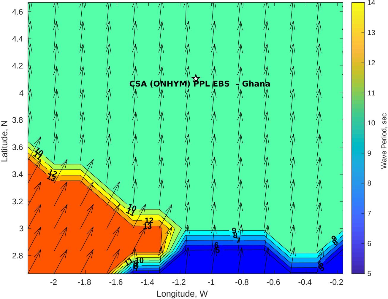
Wave Period (sec) for CSA (ONHYM) PPL EBS - Ghana at 12-Sep-2025 09:00:00
