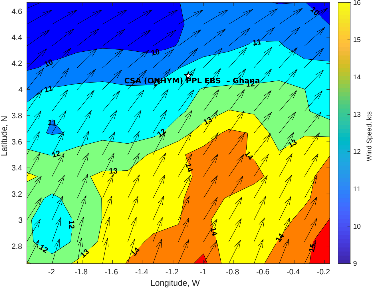
Winds (kts) for CSA (ONHYM) PPL EBS - Ghana at 12-Sep-2025 09:00:00
