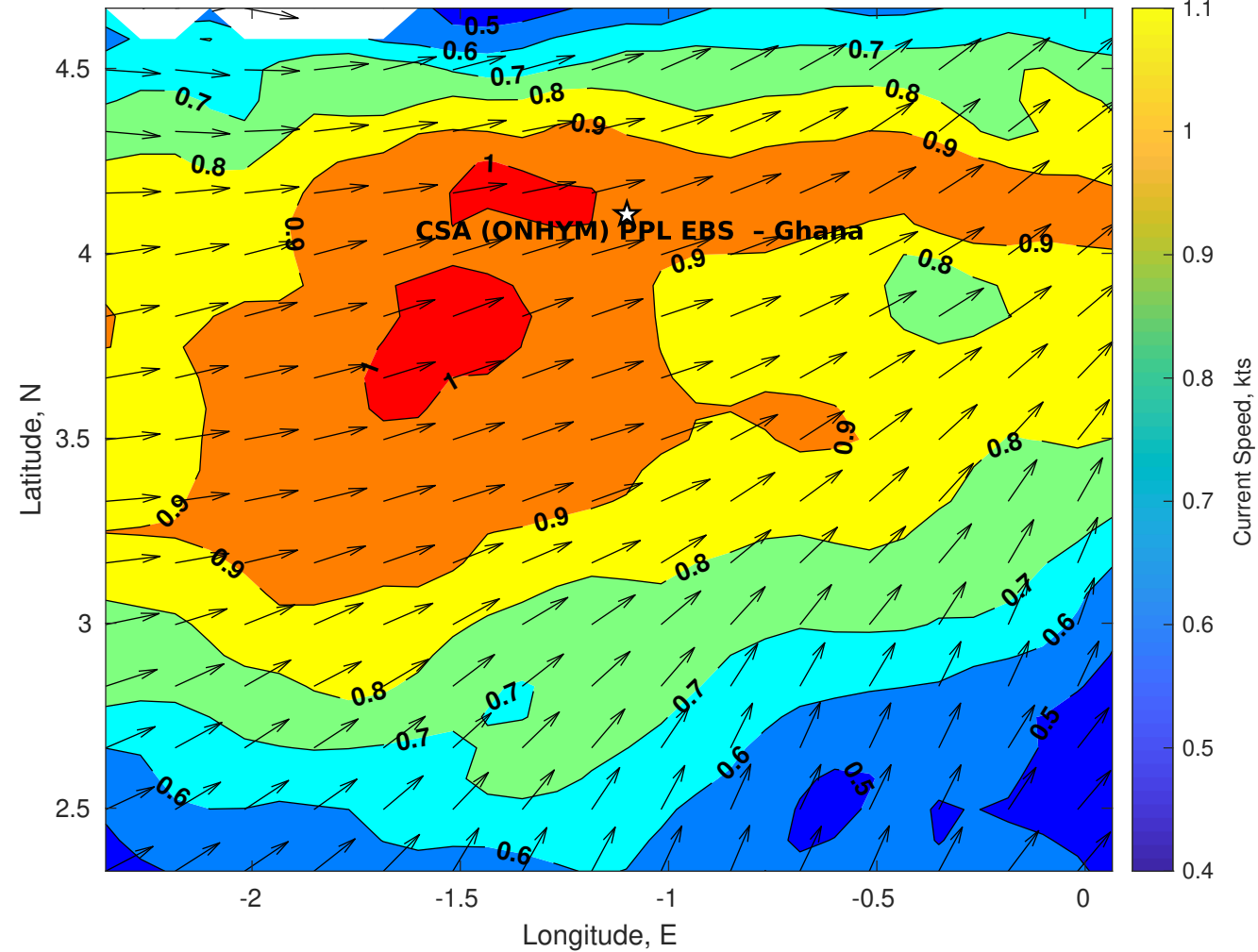
Surface Currents for CSA (ONHYM) PPL EBS - Ghana at 11-Sep-2025 00:00:00
