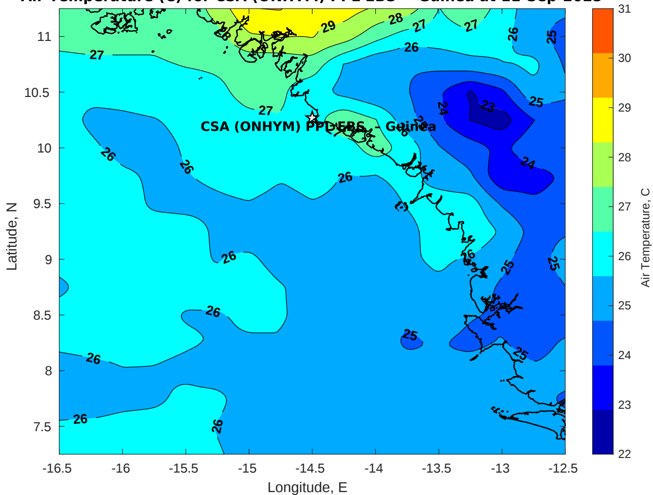
Air Temperature (C) for CSA (ONHYM) PPL EBS - Guinea at 11-Sep-2025
