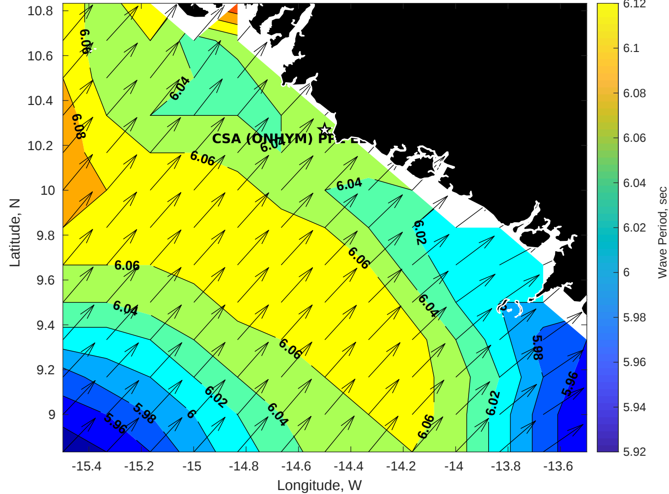
Wave Period (sec) for CSA (ONHYM) PPL EBS - Guinea at 12-Sep-2025 09:00:00
