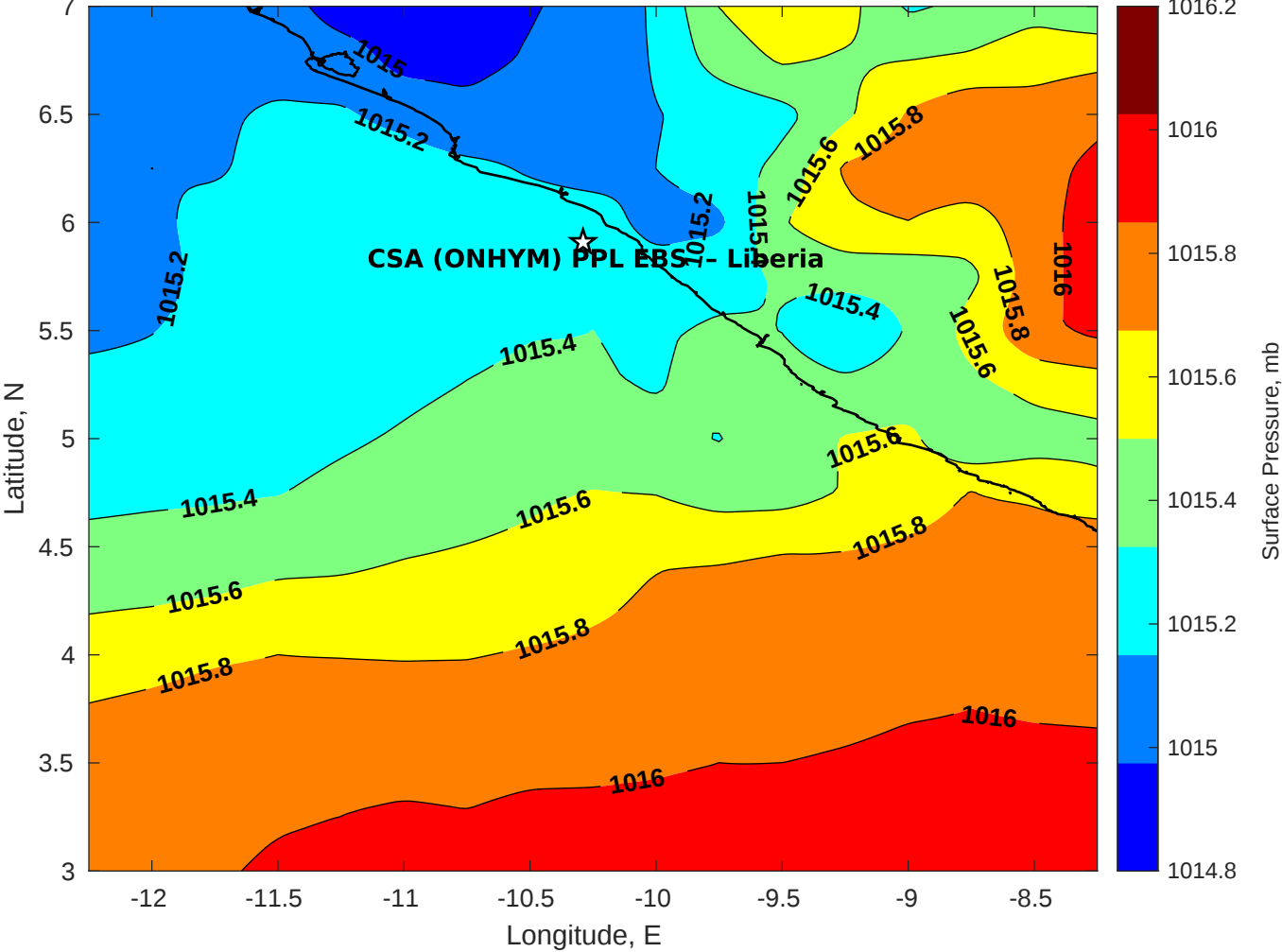
Surface Pressure (mb) for CSA (ONHYM) PPL EBS - Liberia at 13-Sep-2025 12:00:00
