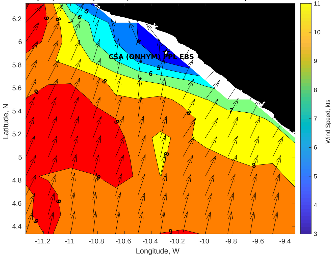
Winds (kts) for CSA (ONHYM) PPL EBS - Liberia at 12-Sep-2025 09:00:00
