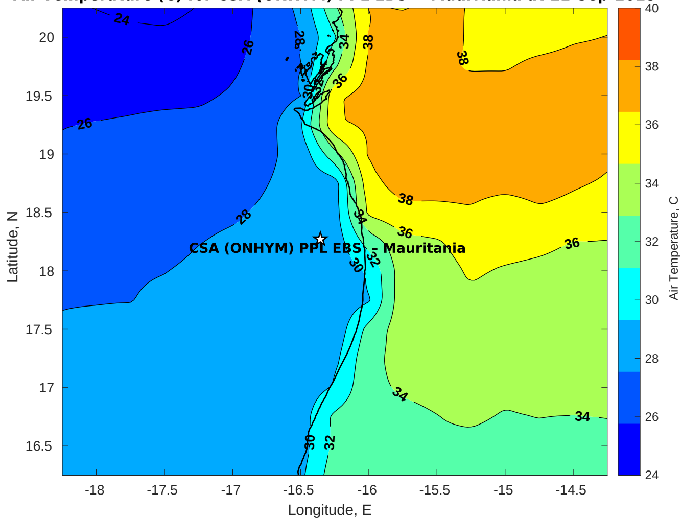
Air Temperature (C) for CSA (ONHYM) PPL EBS - Mauritania at 11-Sep-2025
