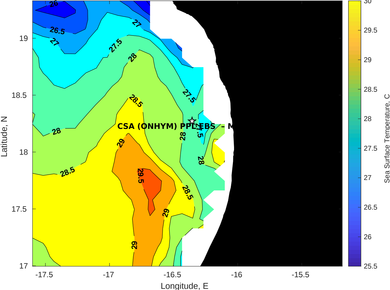
SST for CSA (ONHYM) PPL EBS - Mauritania at 11-Sep-2025 00:00:00
