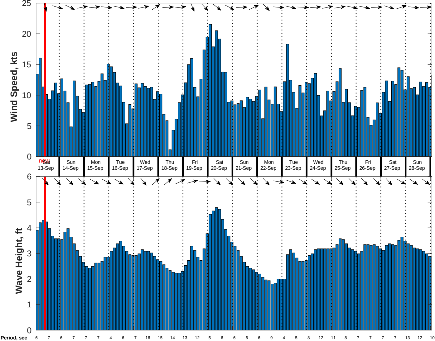
Wind & Wave Forecast for CSA (ONHYM) PPL EBS - Mauritania from 12-Sep-2025 01:00:00 to 28-Sep-2025 01:00:00
