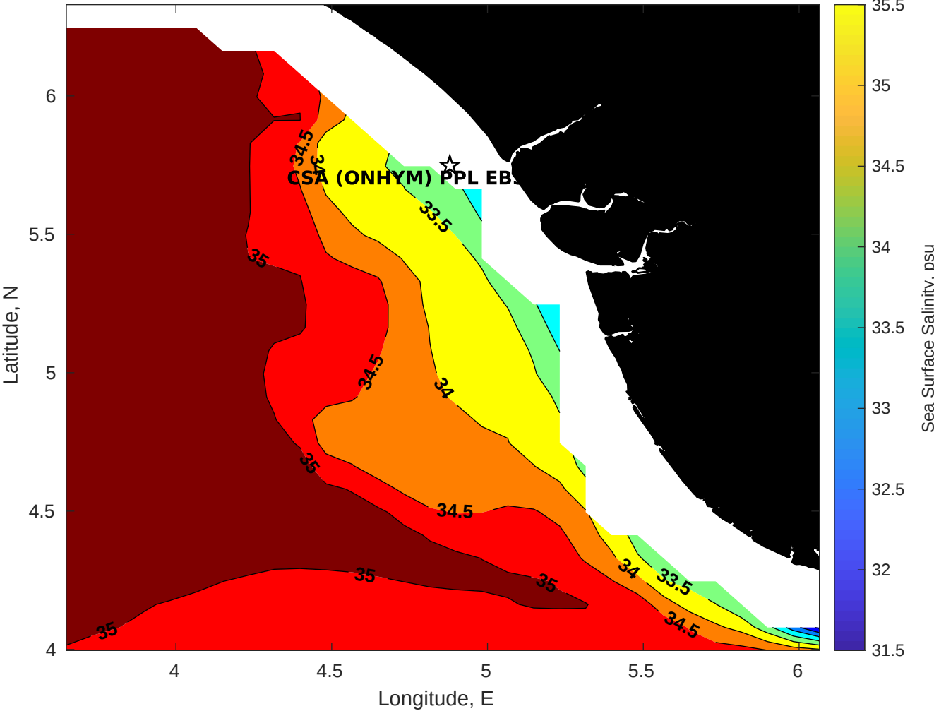
Surface Salinity for CSA (ONHYM) PPL EBS - Nigeria at 11-Sep-2025 00:00:00
