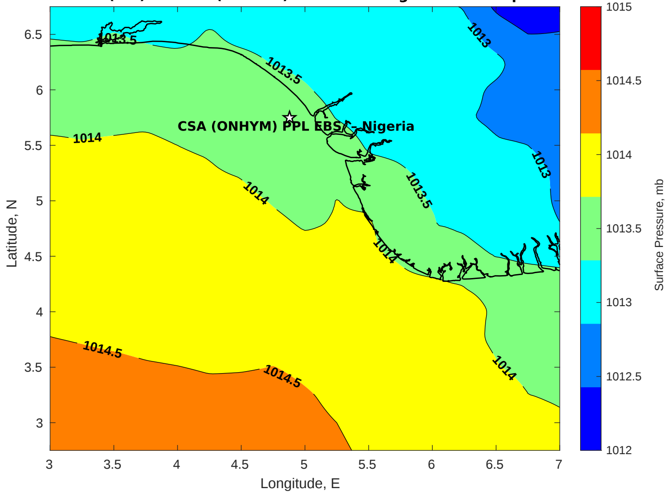
Surface Pressure (mb) for CSA (ONHYM) PPL EBS - Nigeria at 12-Sep-2025 12:00:00
