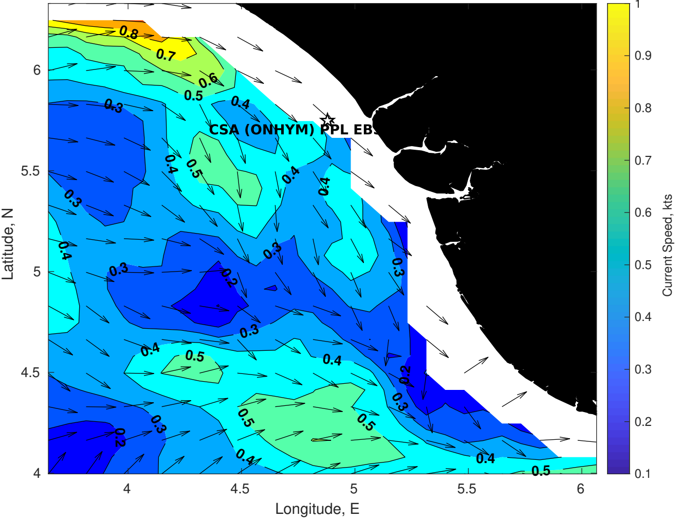
Surface Currents for CSA (ONHYM) PPL EBS - Nigeria at 11-Sep-2025 00:00:00
