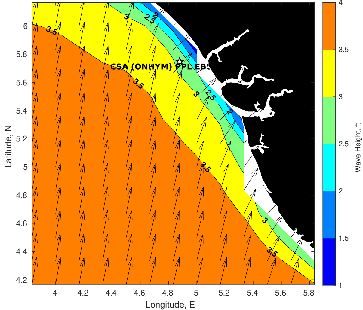
Wave Height (ft) for CSA (ONHYM) PPL EBS - Nigeria at 12-Sep-2025 09:00:00
