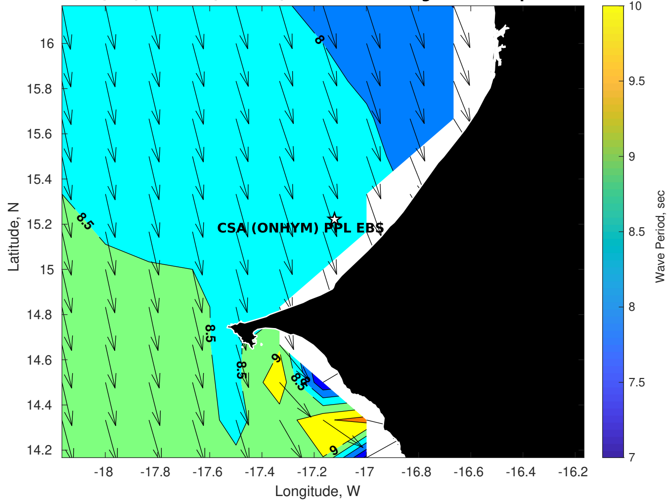
Wave Period (sec) for CSA (ONHYM) PPL EBS - Senegal at 12-Sep-2025 09:00:00
