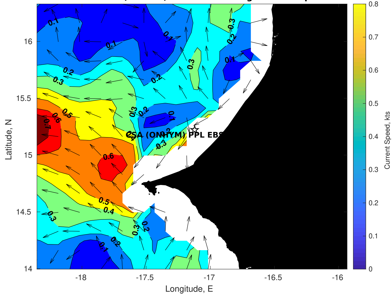
Surface Currents for CSA (ONHYM) PPL EBS - Senegal at 11-Sep-2025 00:00:00
