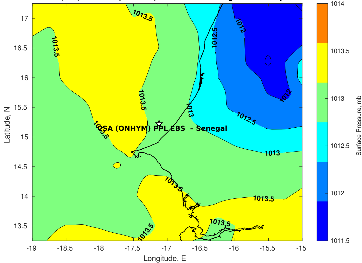
Surface Pressure (mb) for CSA (ONHYM) PPL EBS - Senegal at 13-Sep-2025 12:00:00
