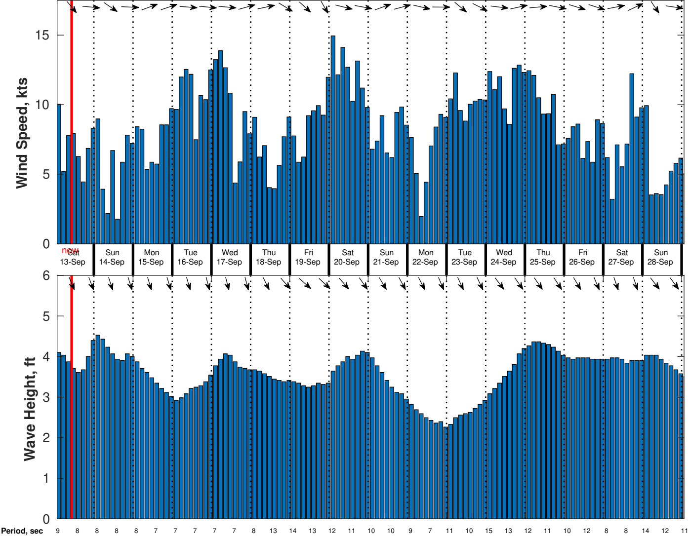
Wind & Wave Forecast for CSA (ONHYM) PPL EBS - Senegal from 12-Sep-2025 01:00:00 to 28-Sep-2025 01:00:00
