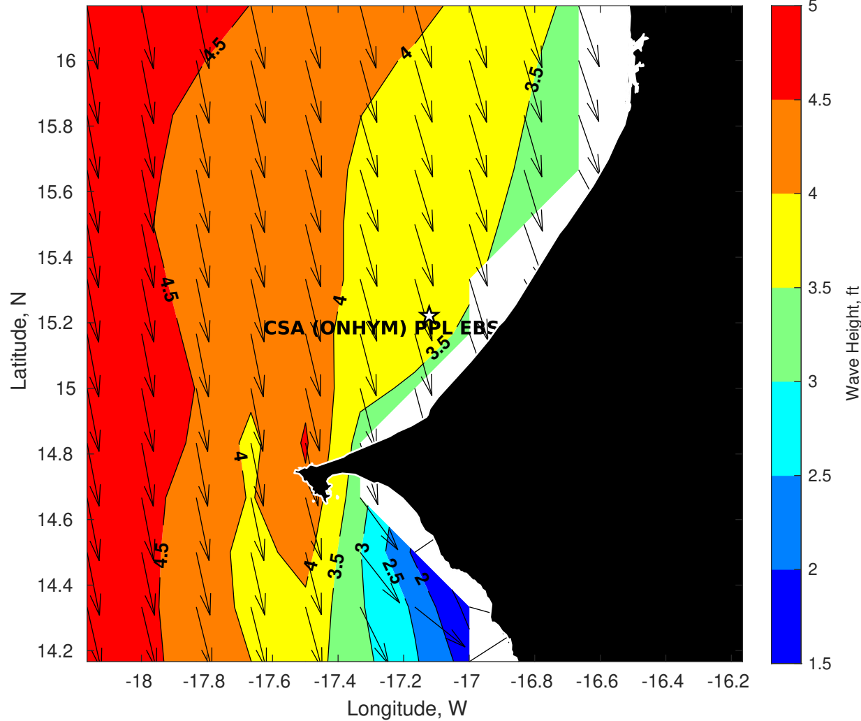
Wave Height (ft) for CSA (ONHYM) PPL EBS - Senegal at 12-Sep-2025 09:00:00
