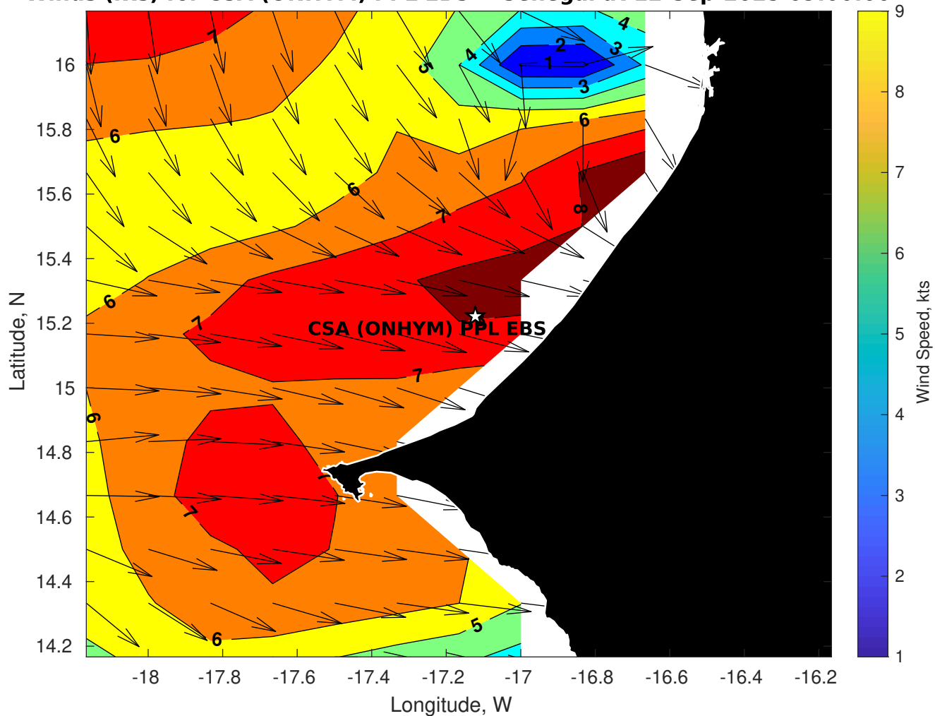
Winds (kts) for CSA (ONHYM) PPL EBS - Senegal at 12-Sep-2025 09:00:00
