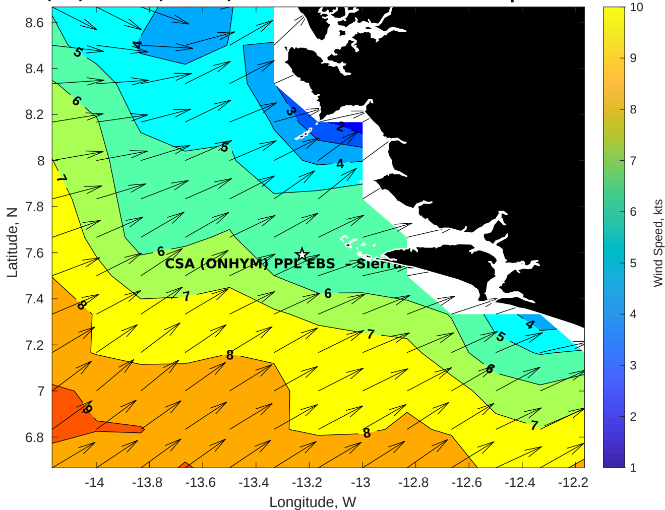
Winds (kts) for CSA (ONHYM) PPL EBS - Sierra Leone at 12-Sep-2025 09:00:00
