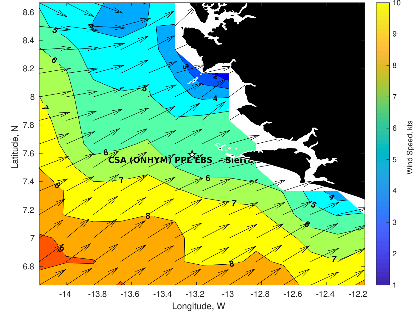
Winds (kts) for CSA (ONHYM) PPL EBS - Sierra Leone at 12-Sep-2025 09:00:00
