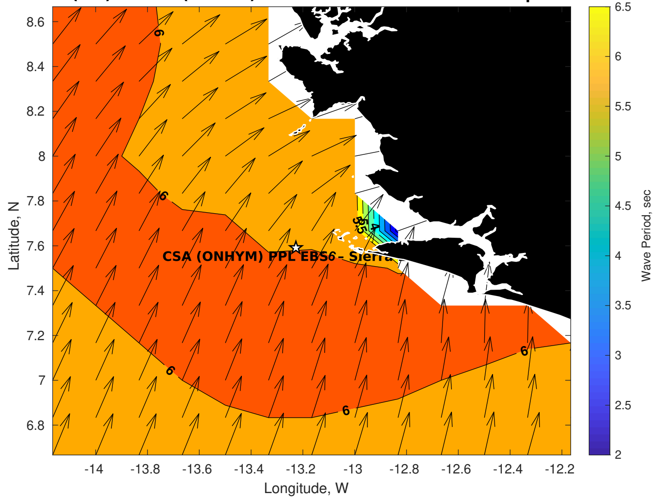
Wave Period (sec) for CSA (ONHYM) PPL EBS - Sierra Leone at 12-Sep-2025 09:00:00
