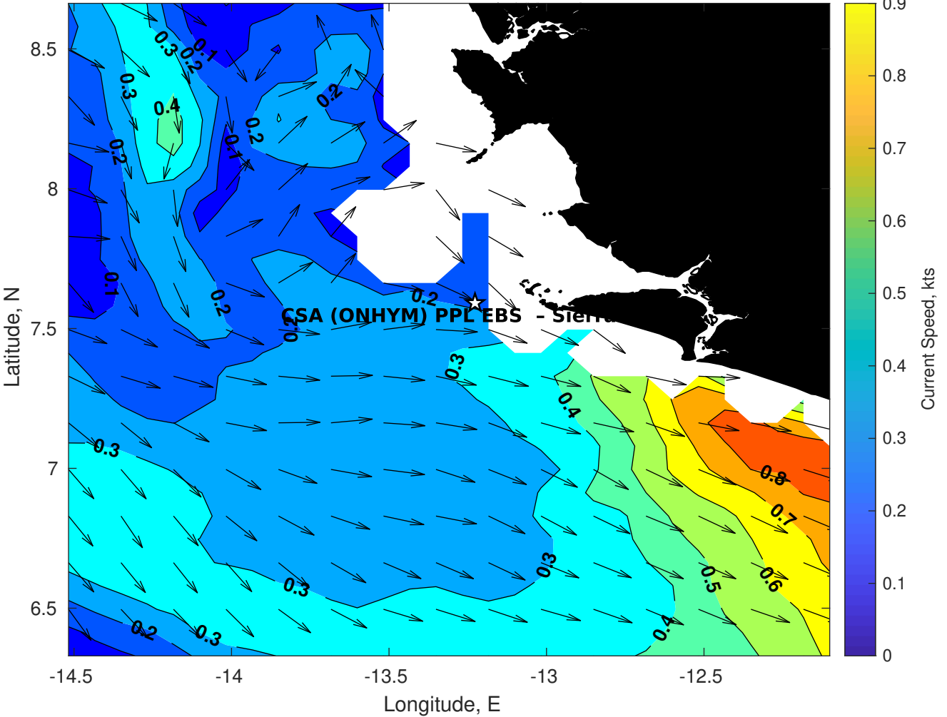
Surface Currents for CSA (ONHYM) PPL EBS - Sierra Leone at 11-Sep-2025 00:00:00
