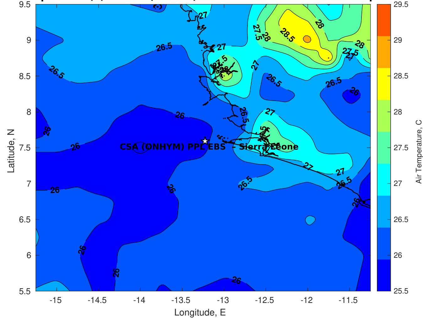
Air Temperature (C) for CSA (ONHYM) PPL EBS - Sierra Leone at 11-Sep-2025
