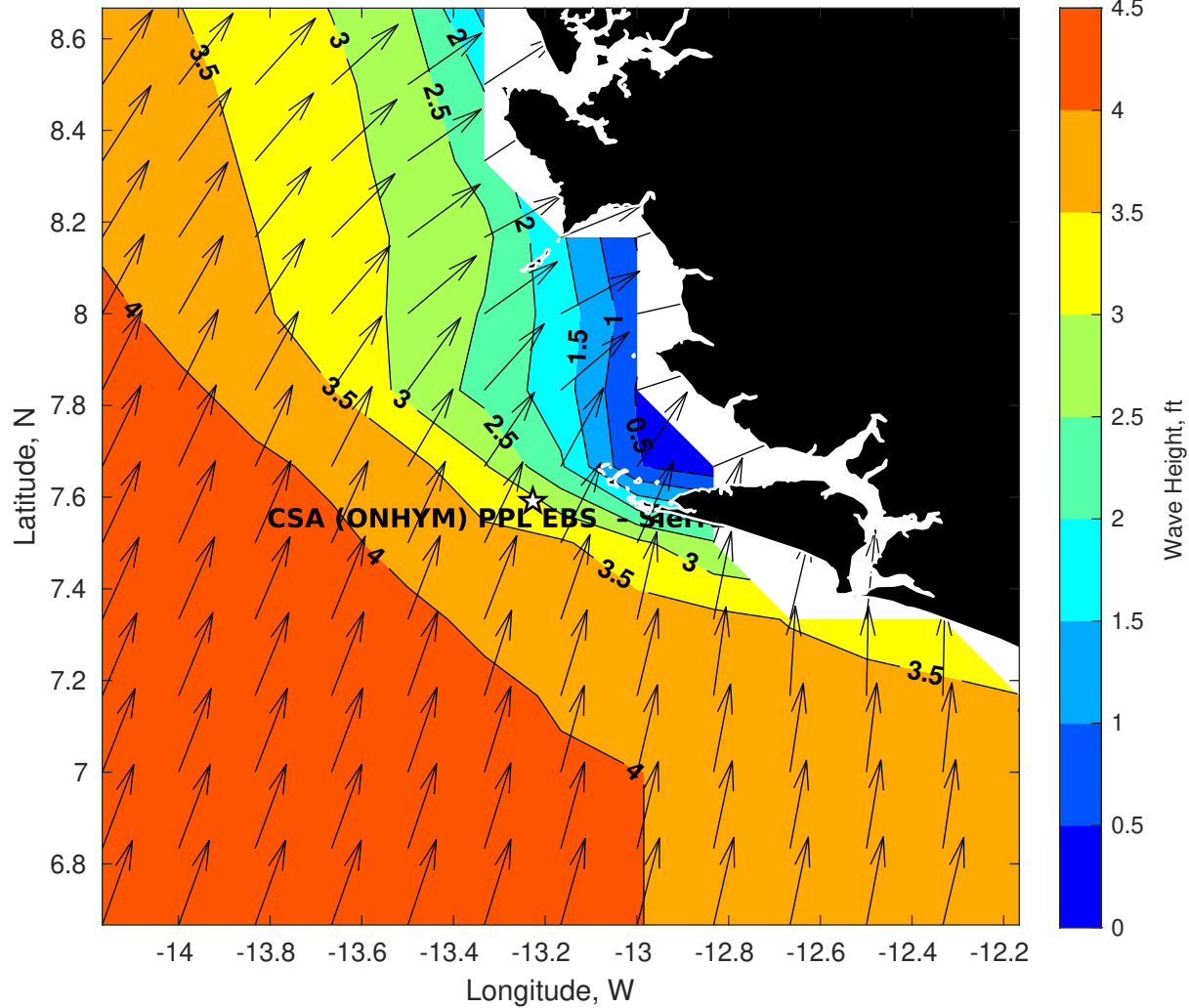
Wave Height (ft) for CSA (ONHYM) PPL EBS - Sierra Leone at 12-Sep-2025 09:00:00
