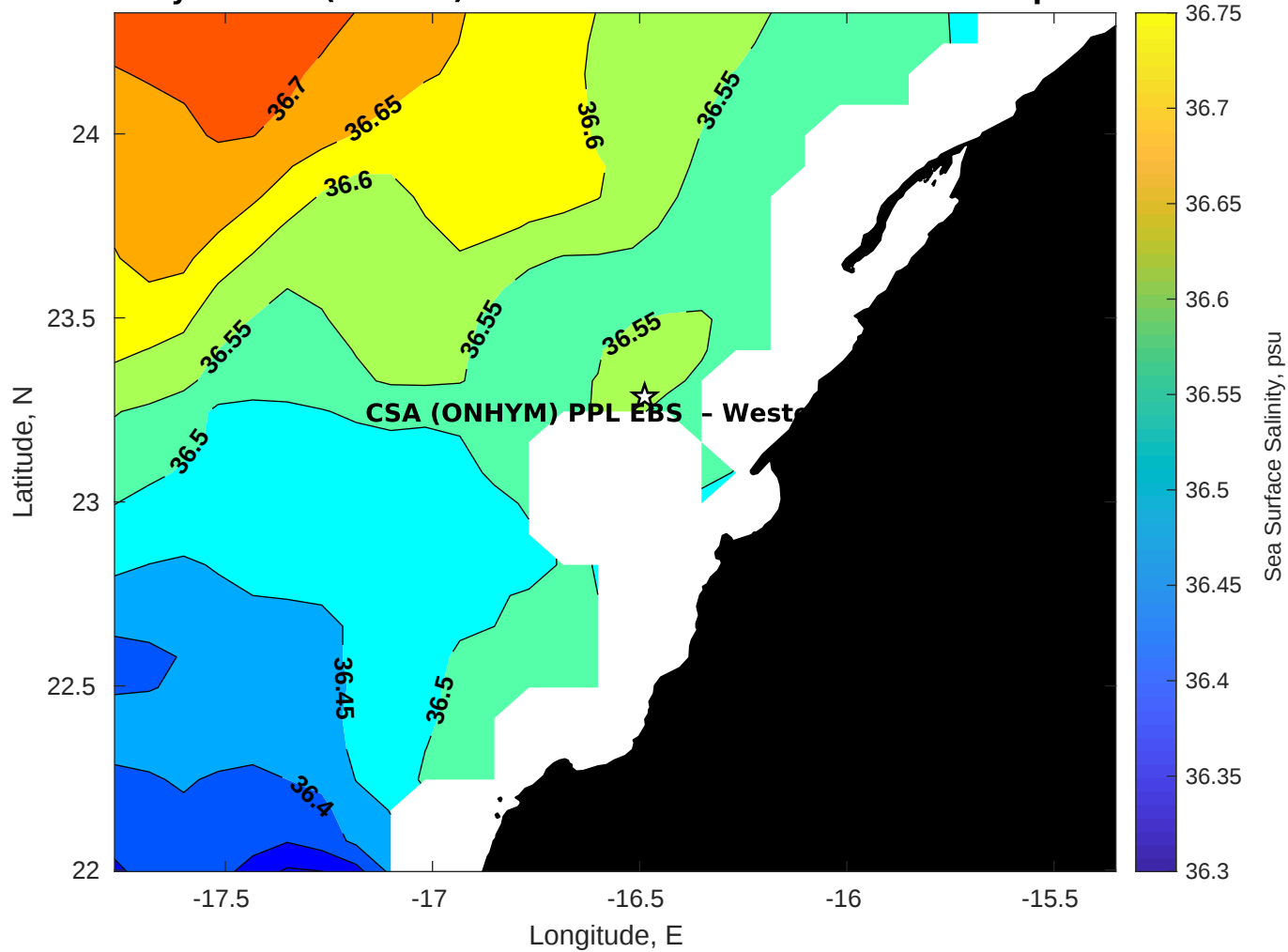
Surface Salinity for CSA (ONHYM) PPL EBS - Western Sahara at 11-Sep-2025 00:00:00
