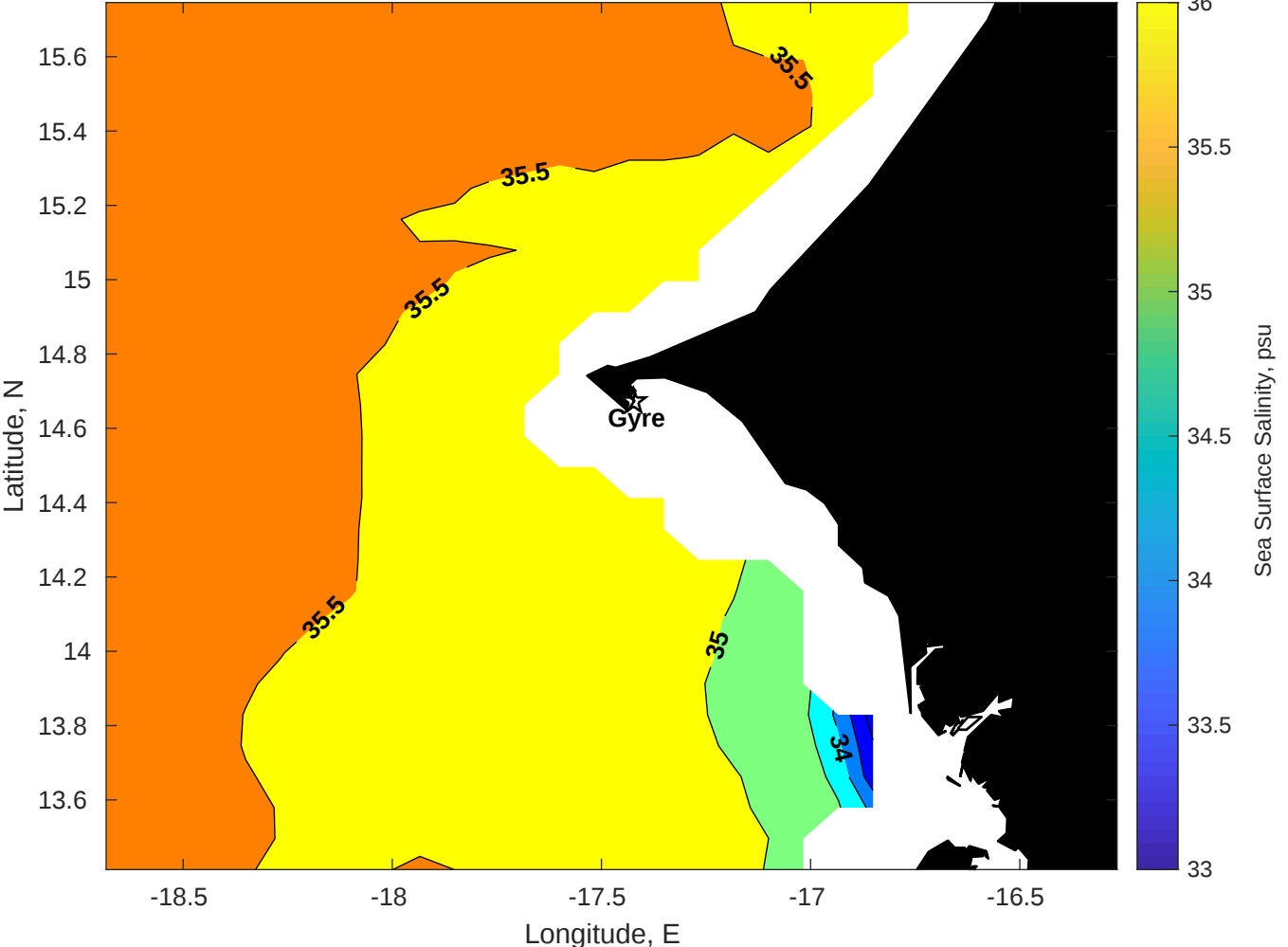
Surface Salinity for Gyre at 11-Sep-2025 00:00:00
