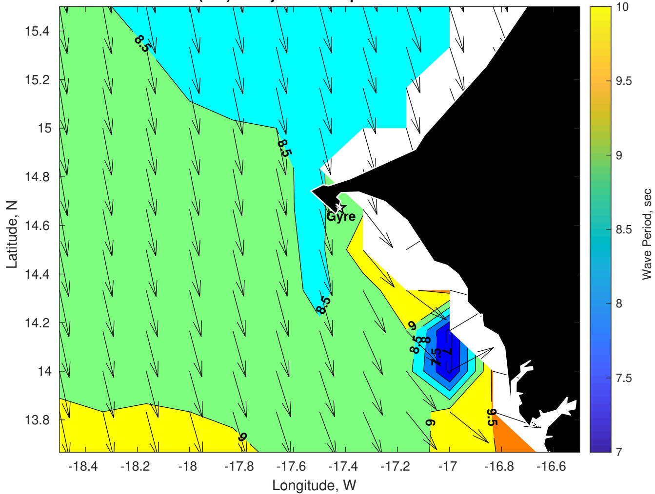
Wave Period (sec) for Gyre at 12-Sep-2025 09:00:00
