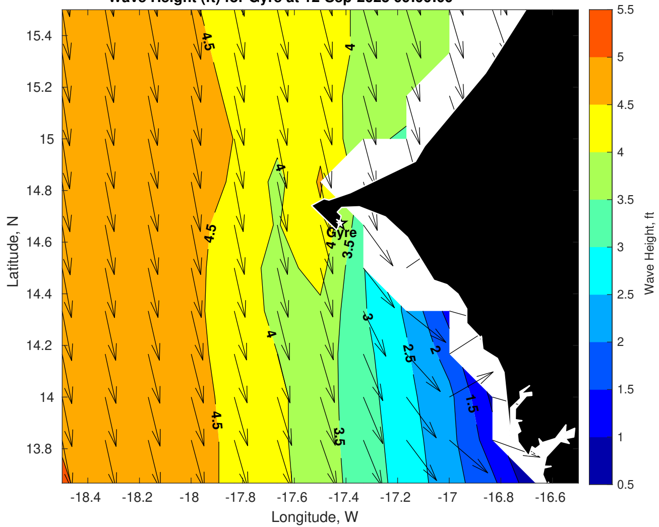
Wave Height (ft) for Gyre at 12-Sep-2025 09:00:00
