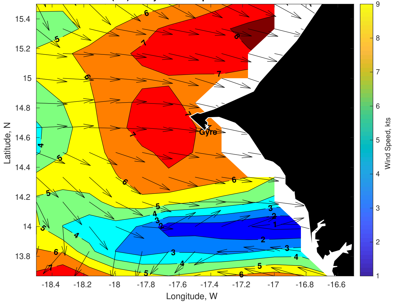
Winds (kts) for Gyre at 12-Sep-2025 09:00:00
