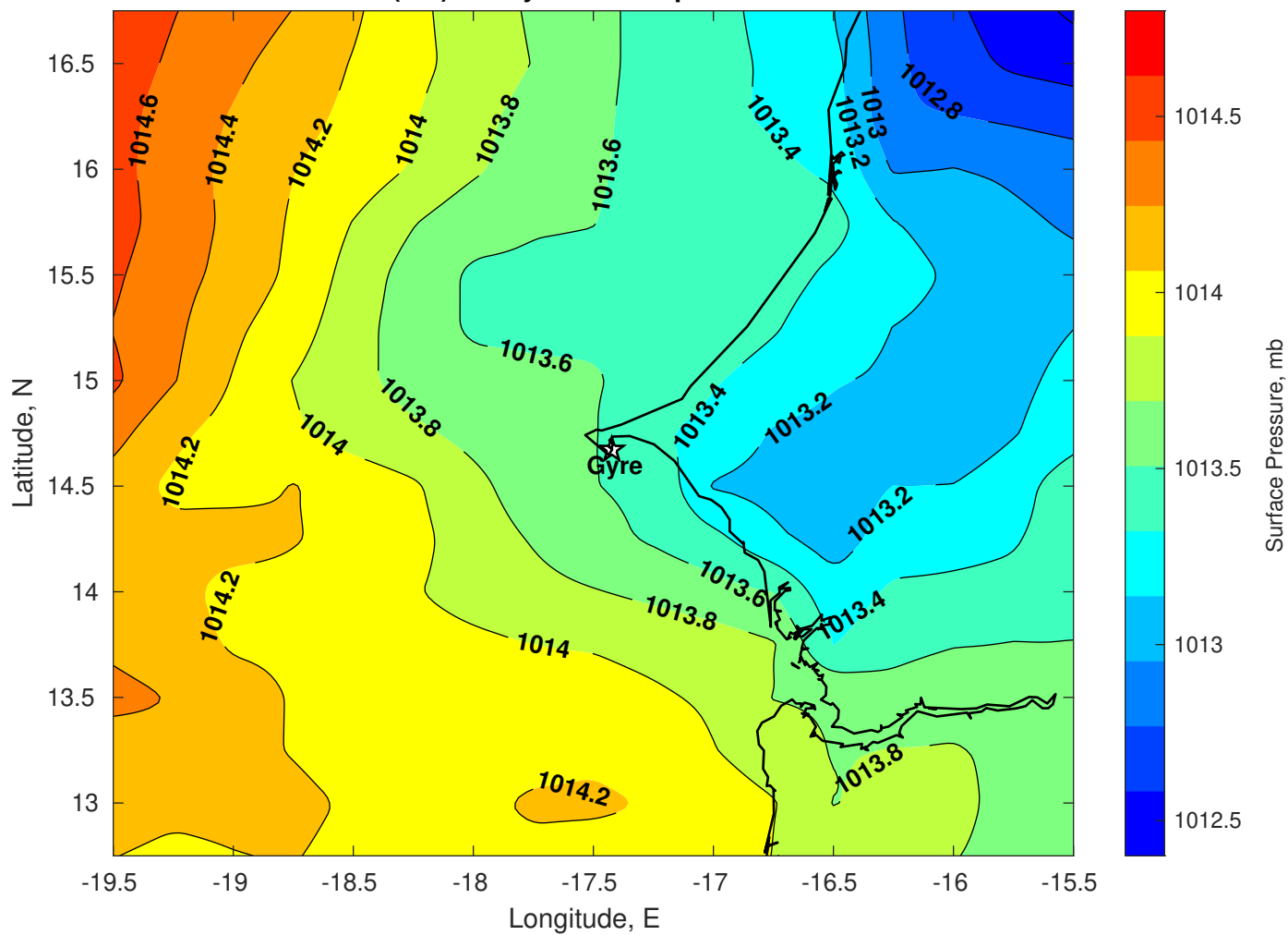
Surface Pressure (mb) for Gyre at 12-Sep-2025 12:00:00
