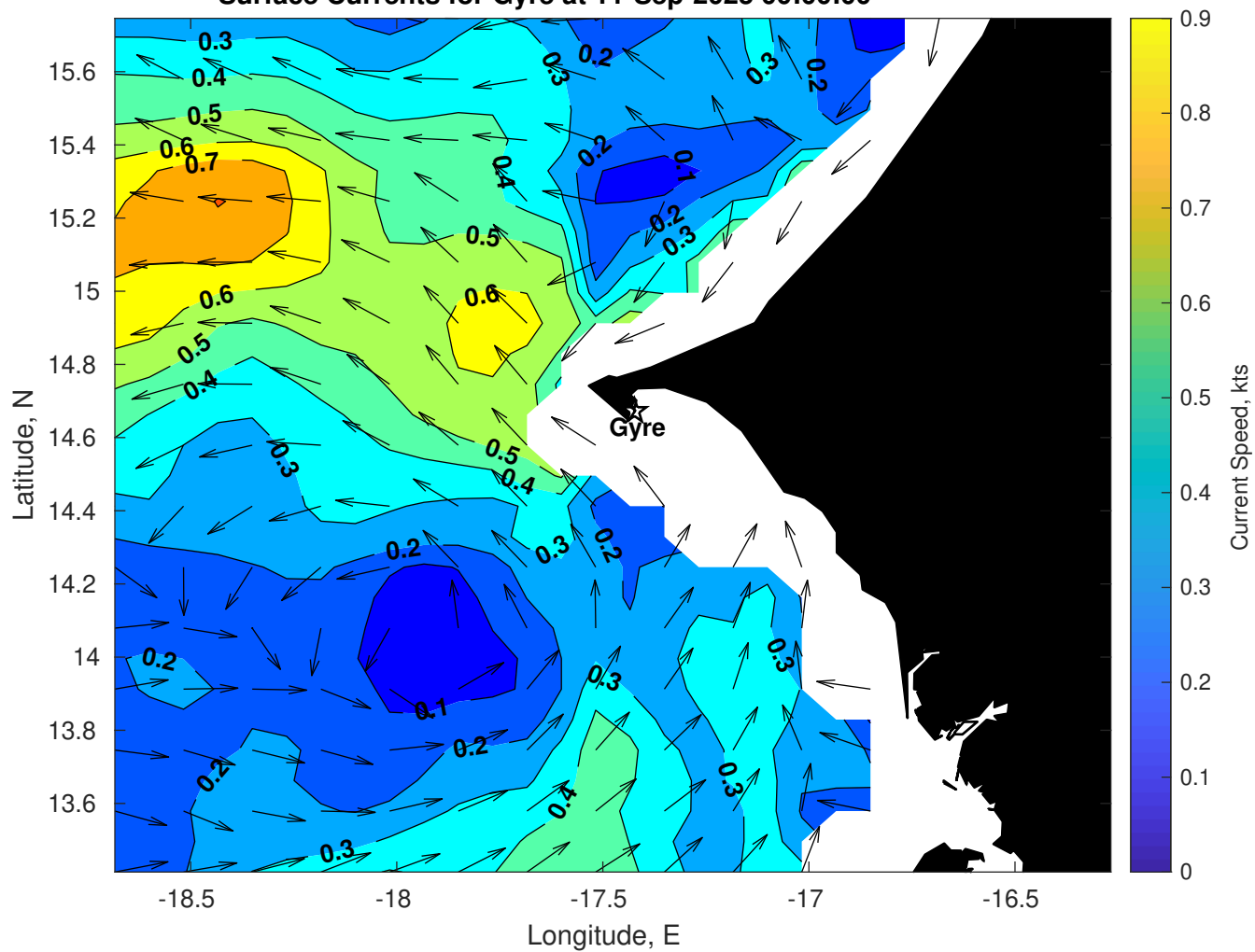
Surface Currents for Gyre at 11-Sep-2025 00:00:00
