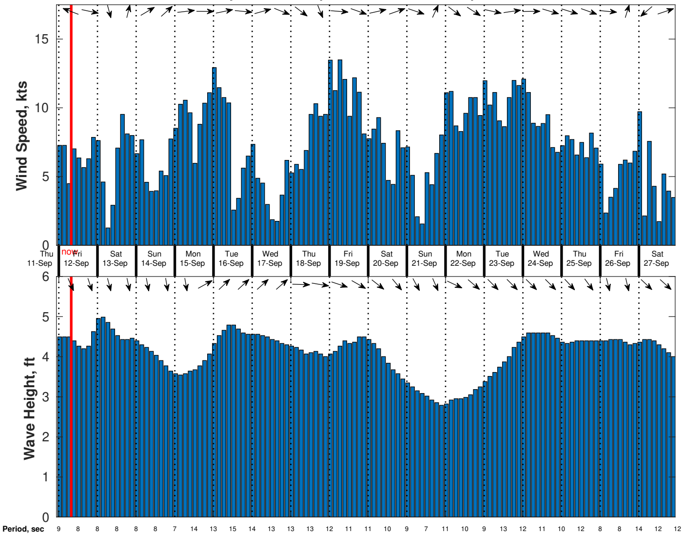
Wind & Wave Forecast for Gyre from 11-Sep-2025 23:00:00 to 27-Sep-2025 23:00:00
