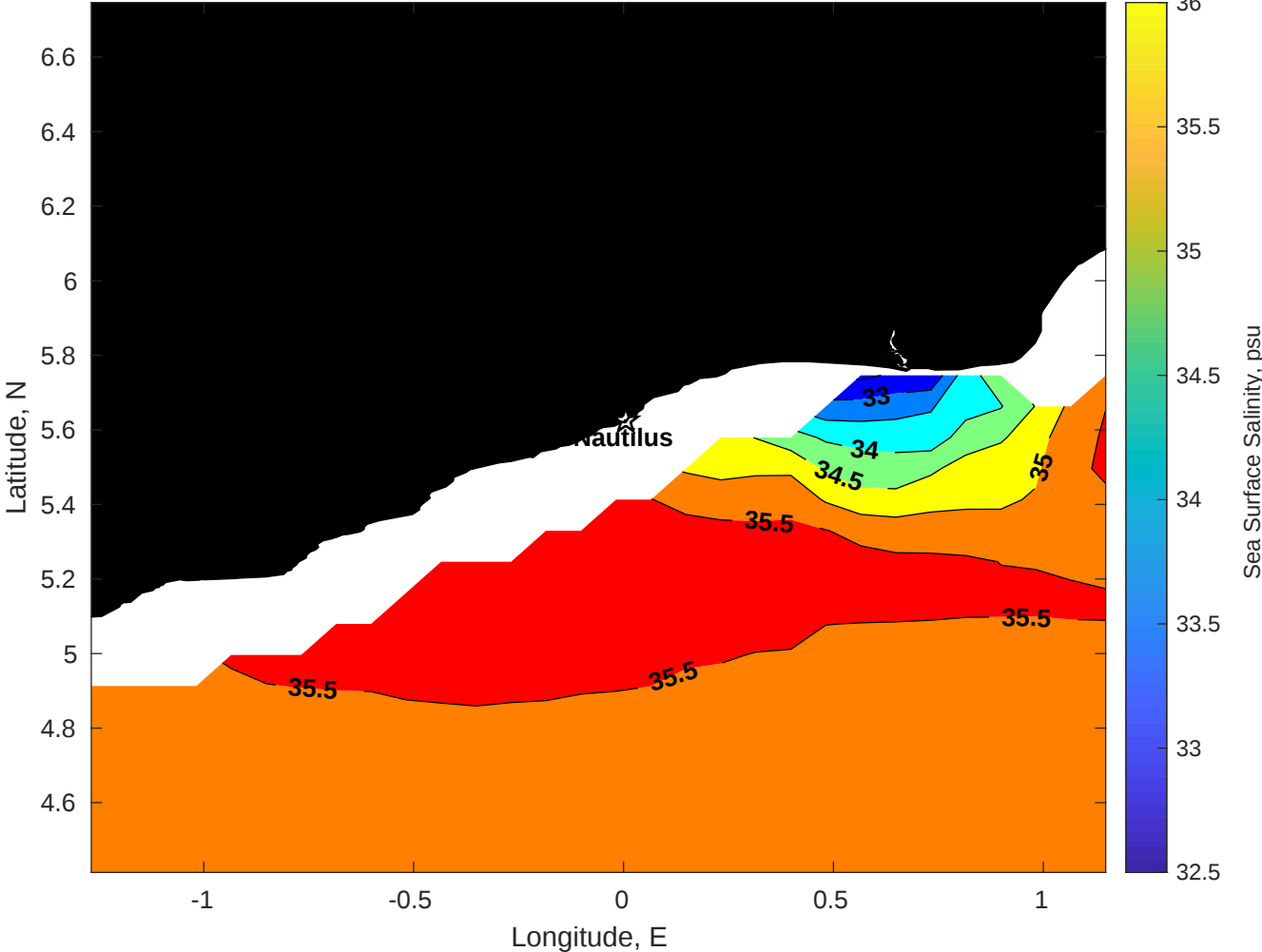
Surface Salinity for Nautilus at 11-Sep-2025 00:00:00
