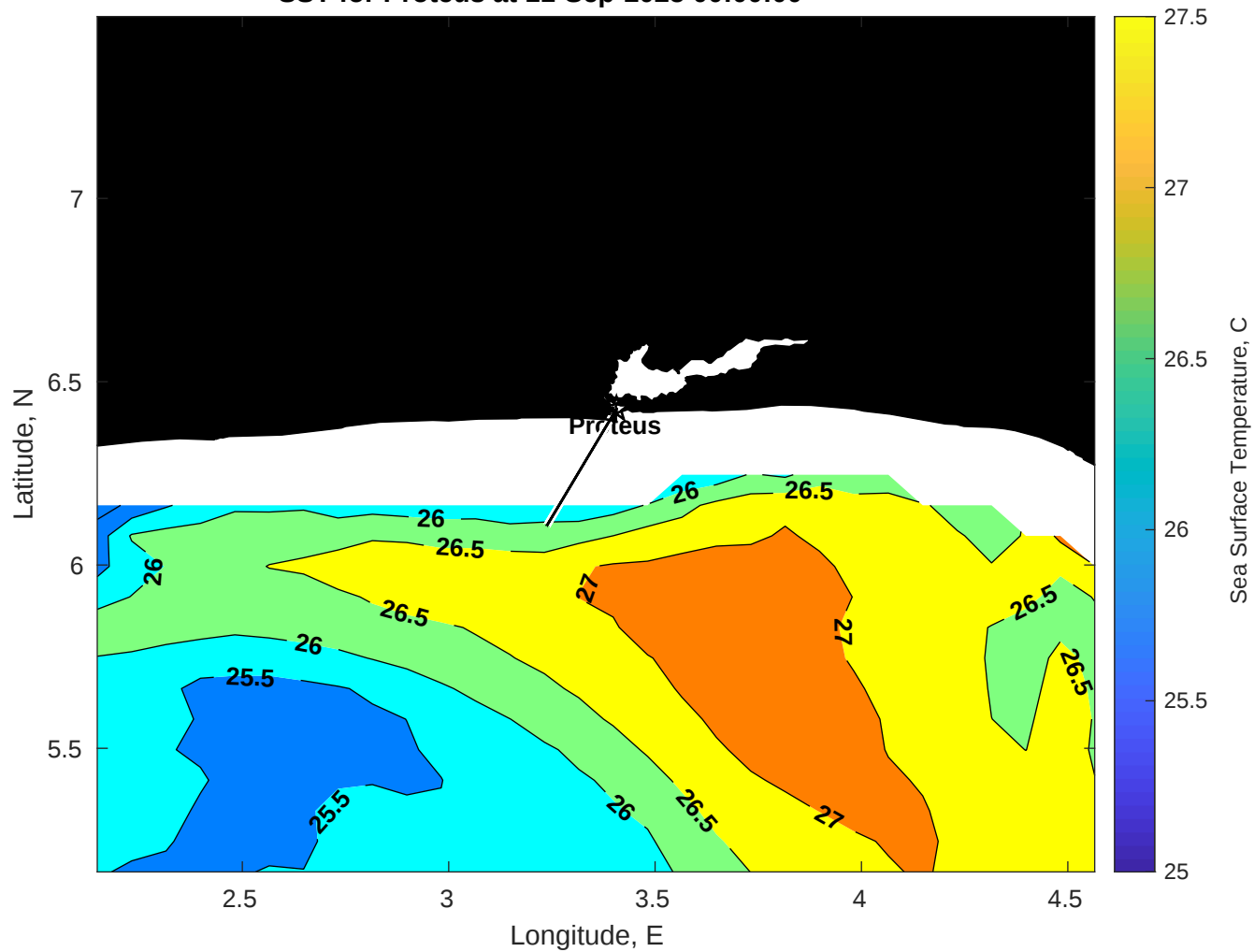
SST for Proteus at 11-Sep-2025 00:00:00
