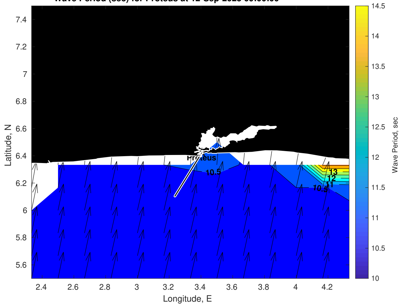
Wave Period (sec) for Proteus at 12-Sep-2025 09:00:00
