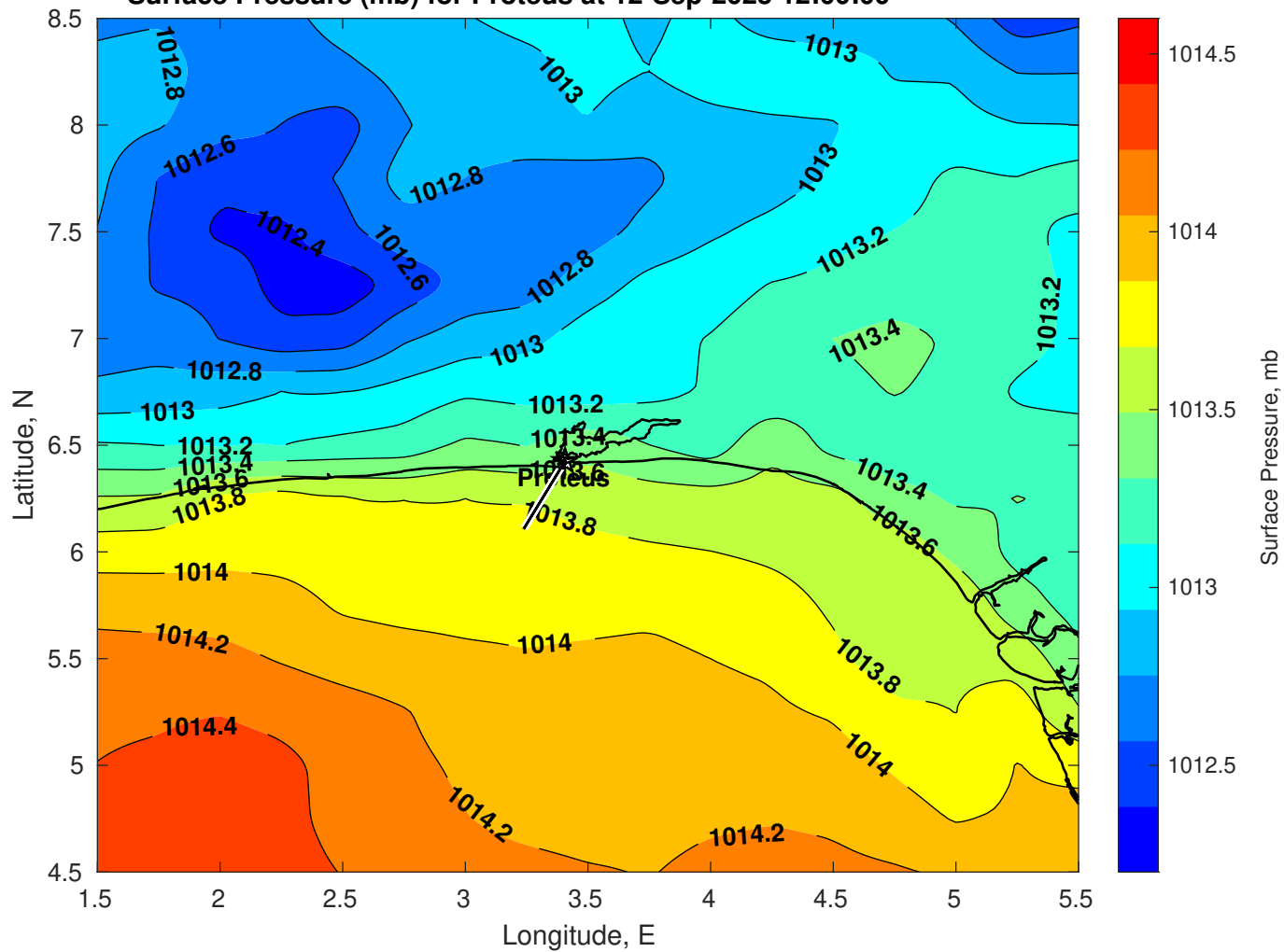
Surface Pressure (mb) for Proteus at 12-Sep-2025 12:00:00
