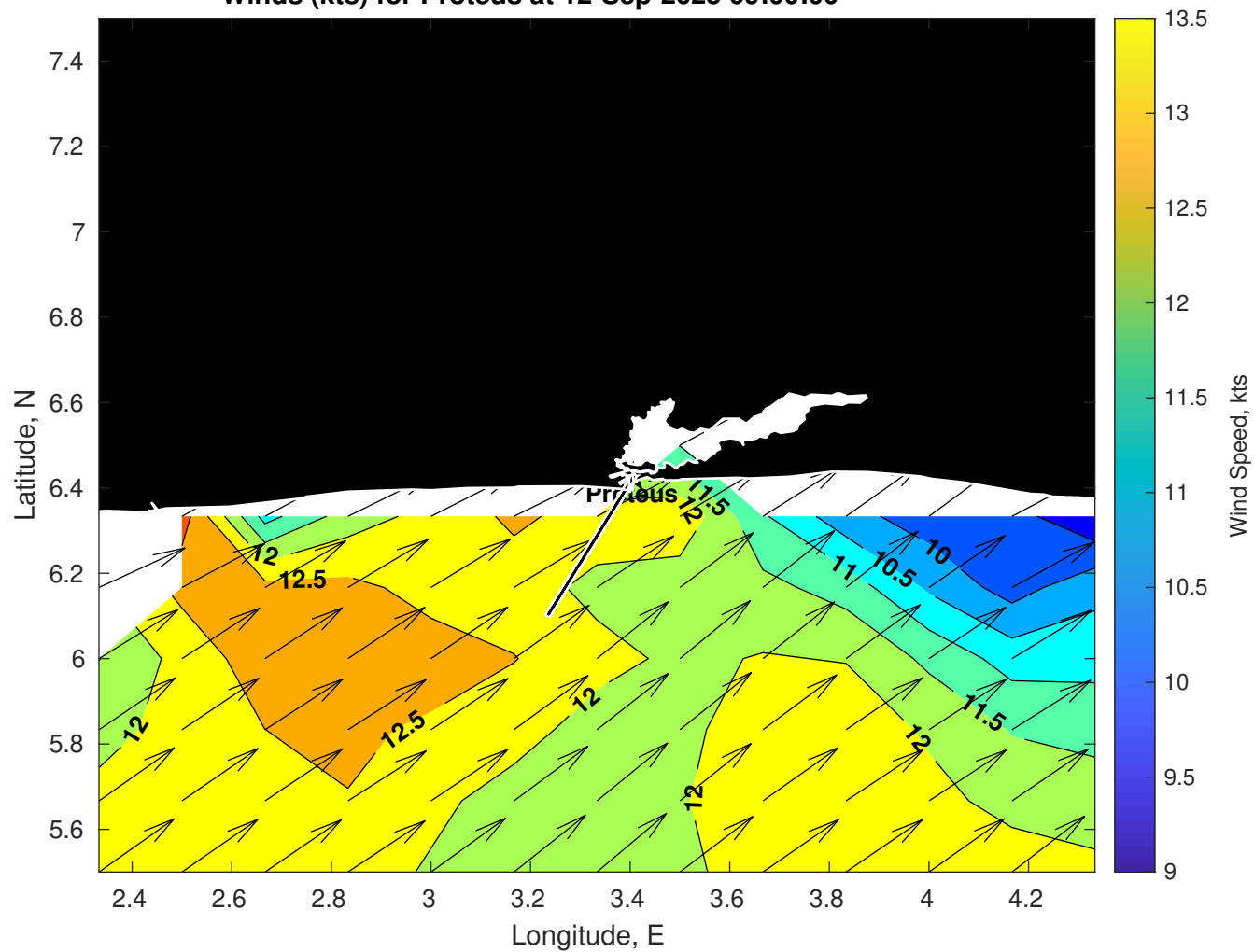
Winds (kts) for Proteus at 12-Sep-2025 09:00:00
