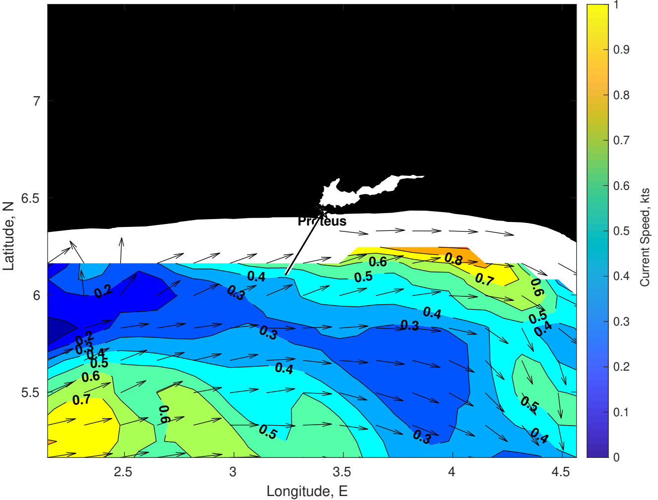
Surface Currents for Proteus at 11-Sep-2025 00:00:00
