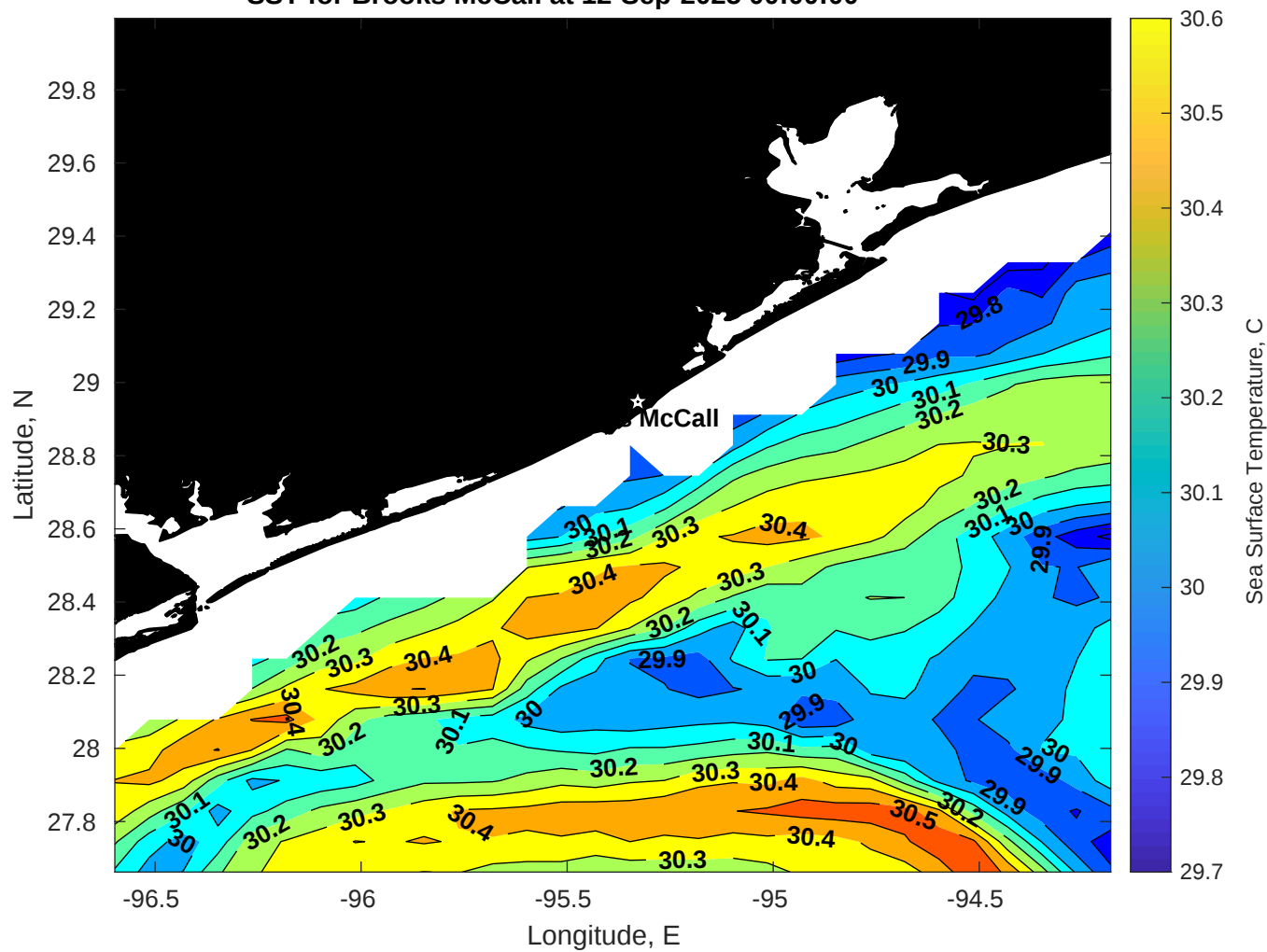
SST for Brooks McCall at 12-Sep-2025 00:00:00
