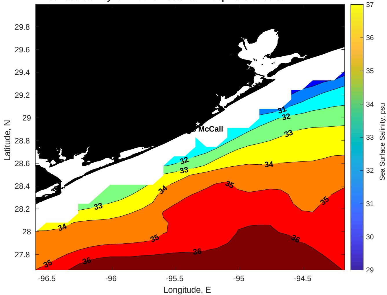
Surface Salinity for Brooks McCall at 12-Sep-2025 00:00:00
