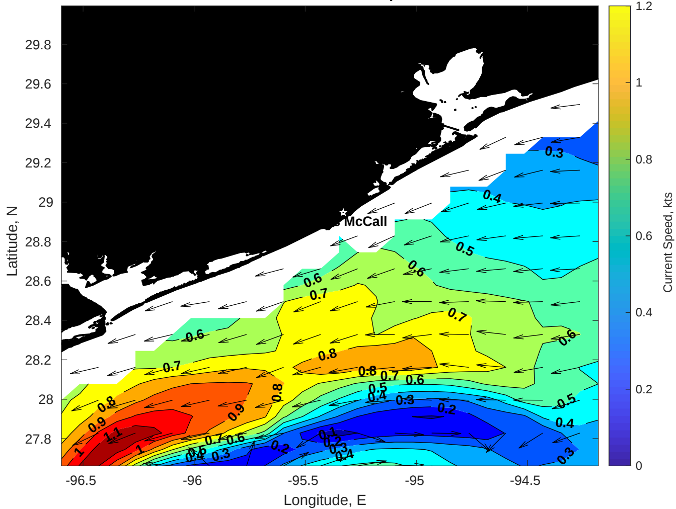
Surface Currents for Brooks McCall at 12-Sep-2025 00:00:00
