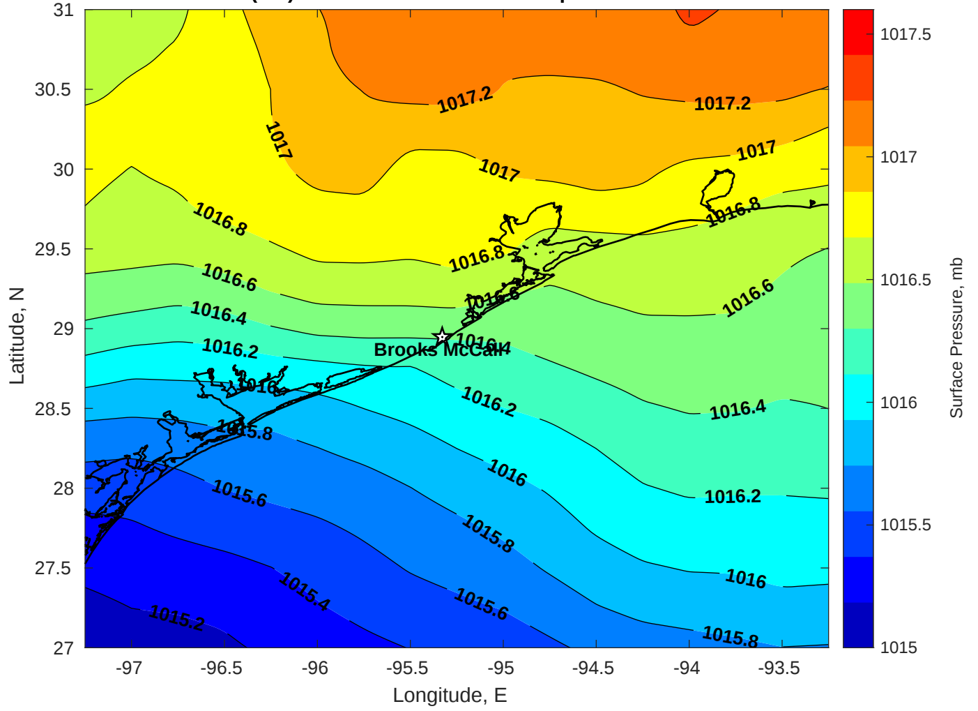
Surface Pressure (mb) for Brooks McCall at 13-Sep-2025 12:00:00
